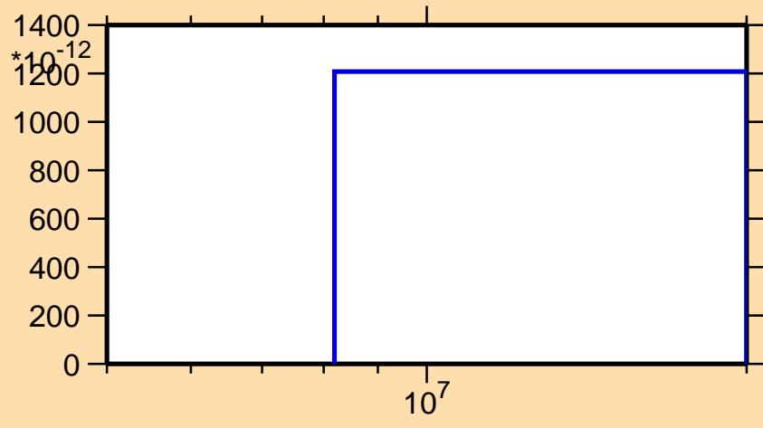
\sigma vs. E for ^{236}\text{Bk} (mt 45)
