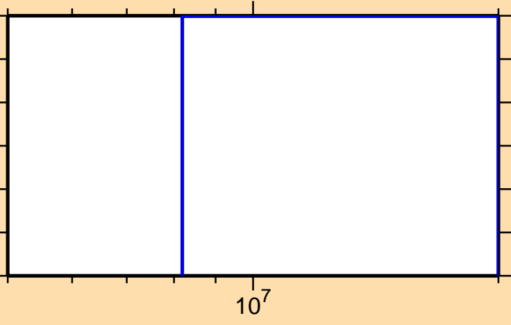
\sigma vs. E for ^{236}\text{Bk}(\text{mt117})
