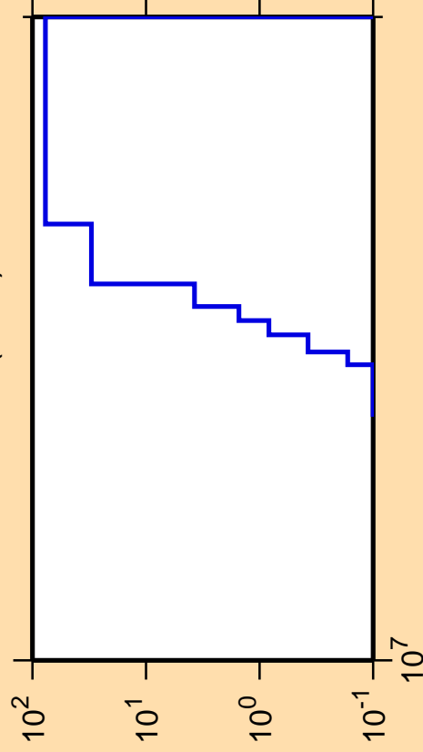
\Delta\sigma/\sigma vs. E for ^{237}\text{Bk}(n,\text{nd})
