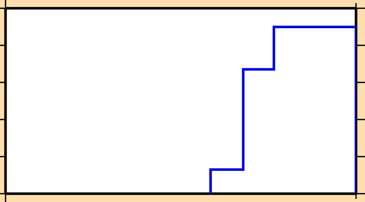
\sigma vs. E for ^{237}\text{Bk}(n,3n\alpha)
