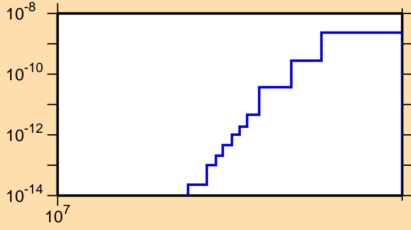
\sigma vs. E for ^{237}\text{Bk}(n,\text{nd})
