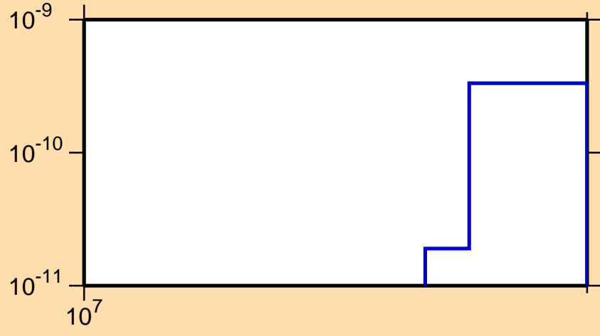
\sigma vs. E for ^{237}\text{Bk}(n,nt)
