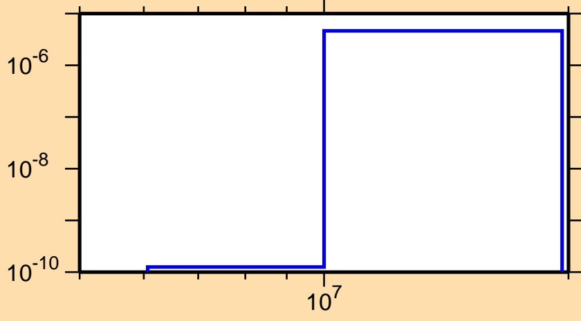
\sigma vs. E for ^{237}\text{Bk}(\text{mt } 45)
