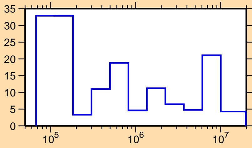
\Delta\sigma/\sigma vs. E for ^{237}\text{Bk}(n,\text{tot.})
