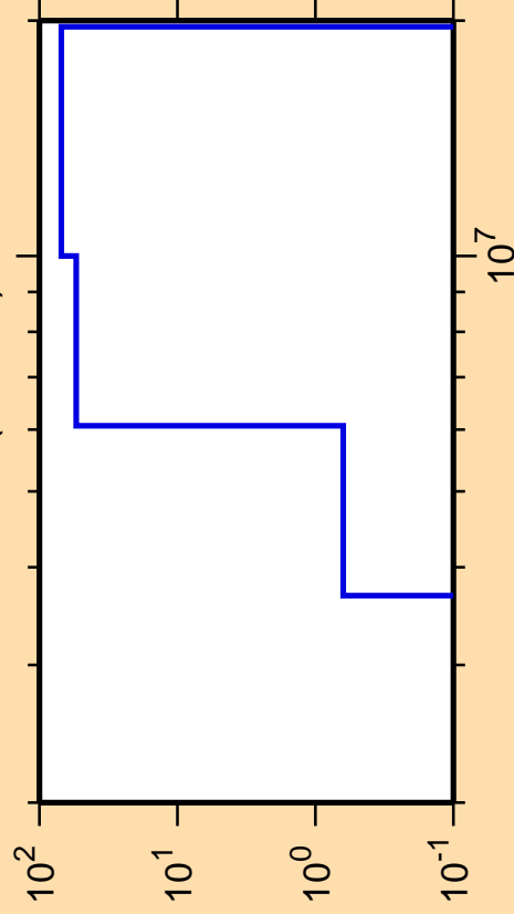
\Delta\sigma/\sigma vs. E for ^{237}\text{Bk}(\text{mt117})
