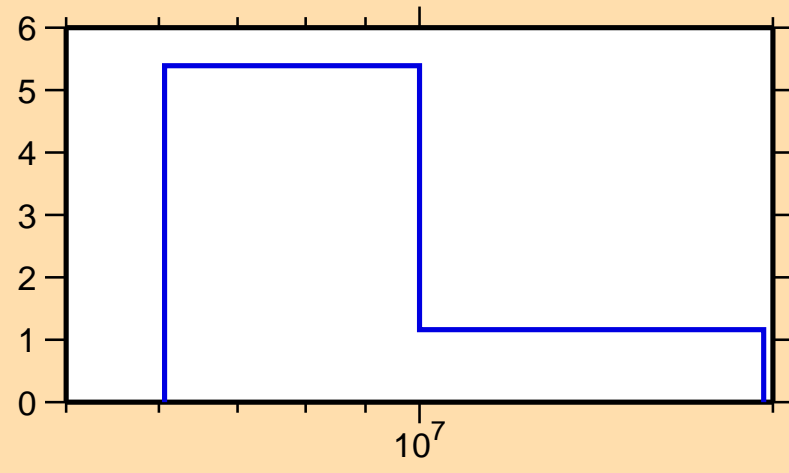
\Delta\sigma/\sigma vs. E for ^{237}\text{Bk}(n,\text{nonel.})
