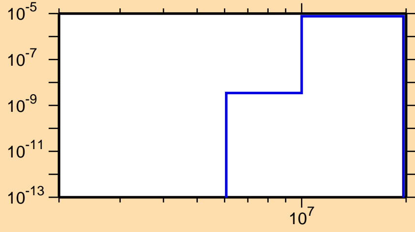
\sigma vs. E for ^{237}\text{Bk}(\text{mt117})
