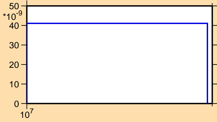
\sigma vs. E for ^{237}\text{Bk}(n,3n\alpha)
