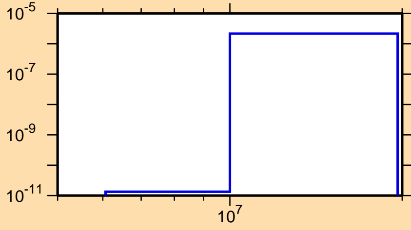
\sigma vs. E for ^{237}\text{Bk}(n,t)
