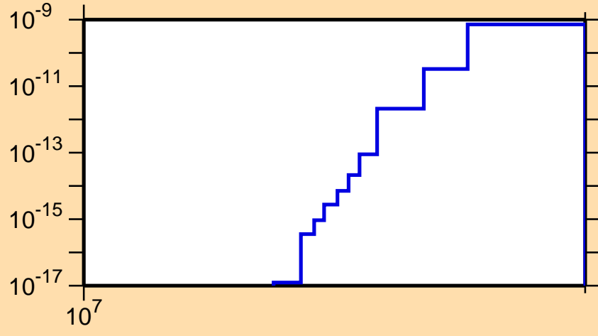
\sigma vs. E for ^{238}\text{Bk}(n,nt)
