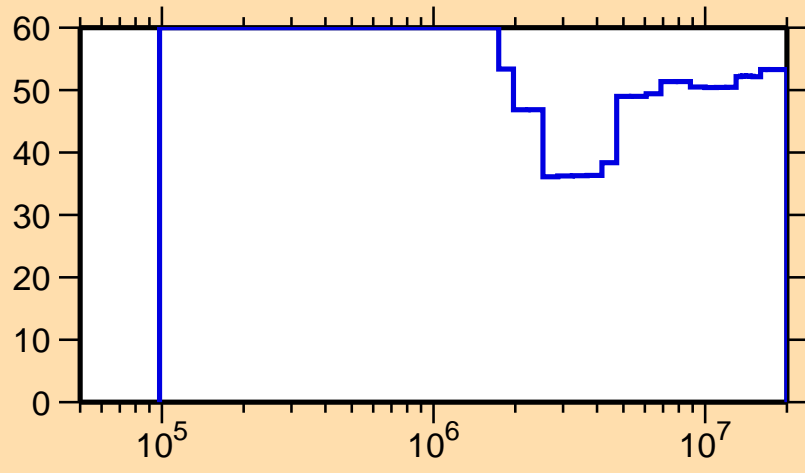
\Delta\sigma/\sigma vs. E for ^{238}\text{Bk}(n,n_1)
