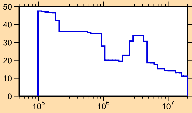
\Delta\sigma/\sigma vs. E for ^{238}\text{Bk}(n,f)
