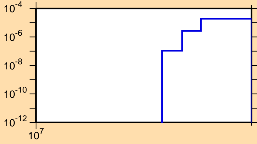
\sigma vs. E for ^{238}\text{Bk}(n,3n\alpha)
