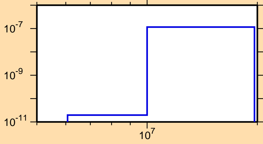
\sigma vs. E for ^{238}\text{Bk}(\text{mt117})
