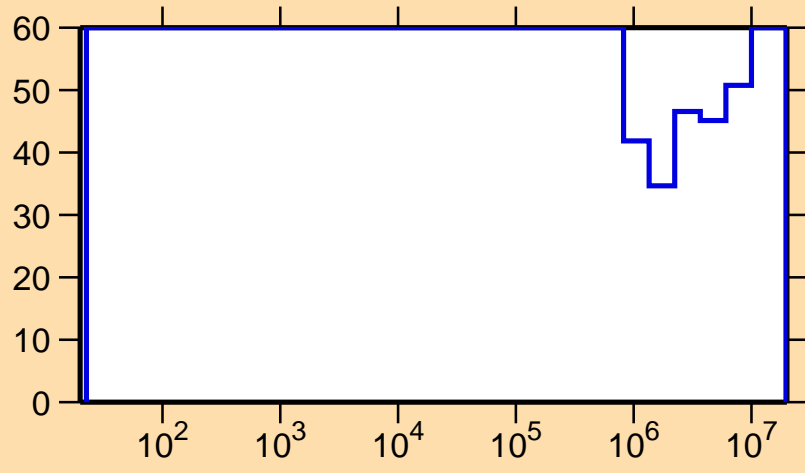
\Delta\sigma/\sigma vs. E for ^{238}\text{Bk}(n,p)
