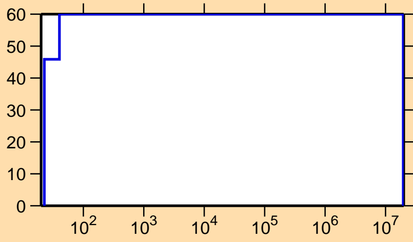
\Delta\sigma/\sigma vs. E for ^{238}\text{Bk}(n,\gamma)
