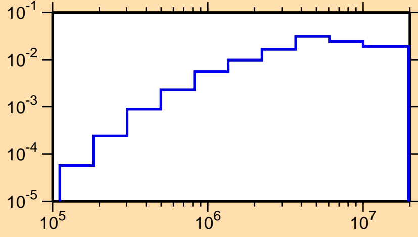
\sigma vs. E for ^{238}\text{Bk}(n,n\alpha)
