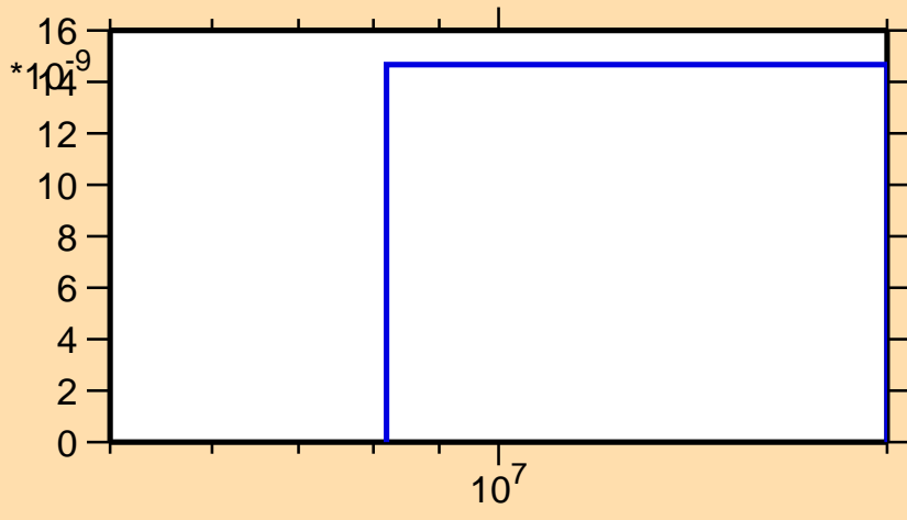
\sigma vs. E for ^{238}\text{Bk}(n,\text{He3})
