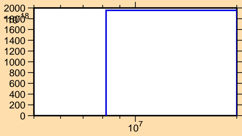
\sigma vs. E for ^{238}\text{Bk}(\text{mt } 34)
