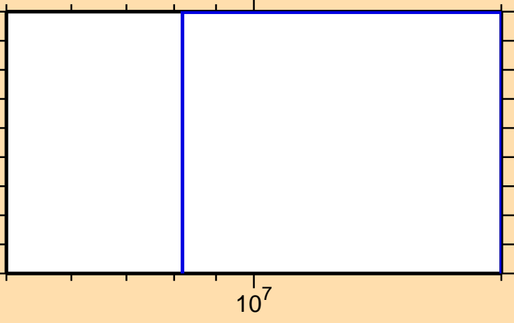
\sigma vs. E for ^{238}\text{Bk}(n,3n)
