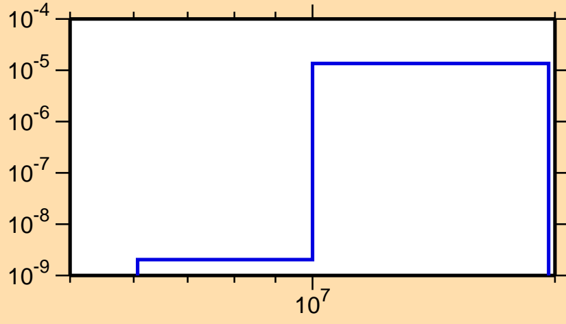
\sigma vs. E for ^{239}\text{Bk}(\text{mt117})
