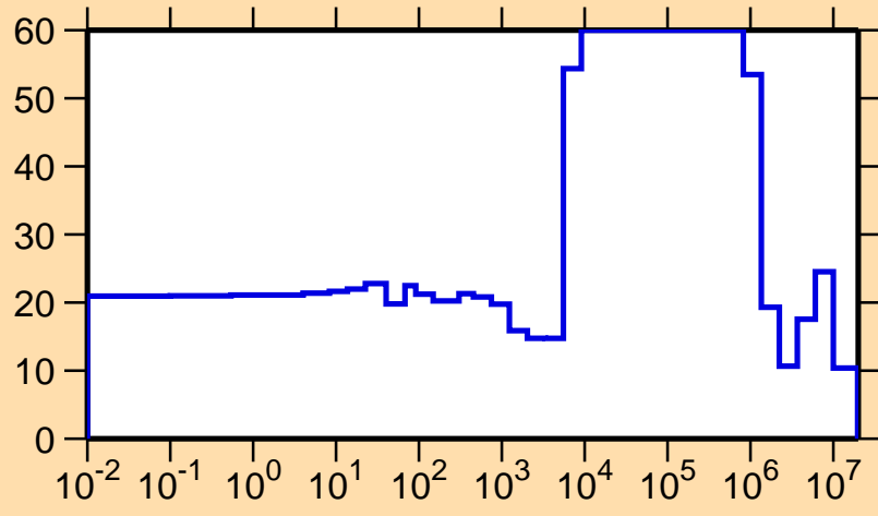
\Delta\sigma/\sigma vs. E for ^{239}\text{Bk}(n,el.)
