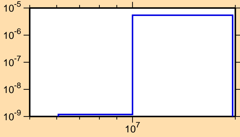
\sigma vs. E for ^{239}\text{Bk} (mt 45)
