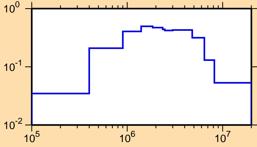
\sigma vs. E for ^{239}\text{Bk}(n,n\text{cont.})
