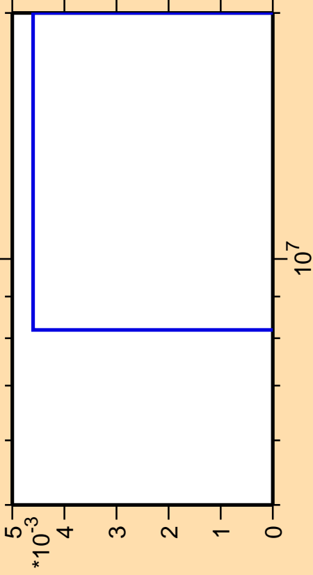
\Delta\sigma/\sigma vs. E for ^{239}\text{Bk} (mt 34)
