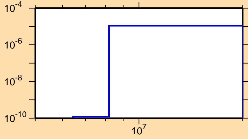
\sigma vs. E for ^{239}\text{Bk}(\text{mt117})
