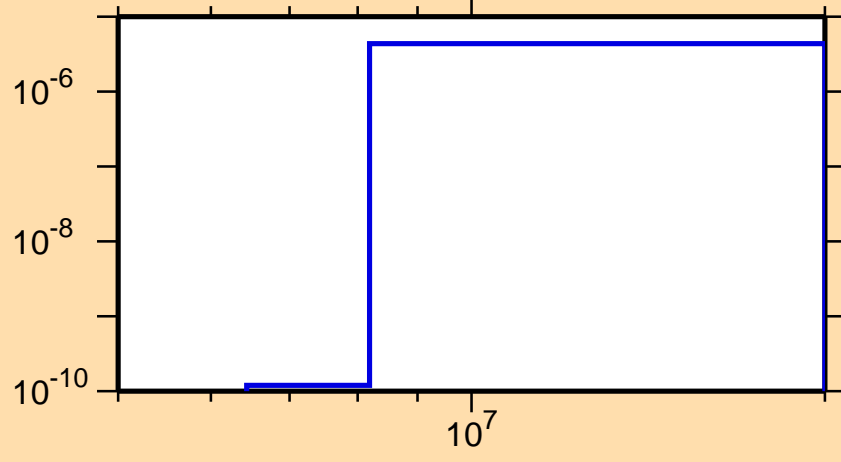
\sigma vs. E for ^{239}\text{Bk} (mt 45)
