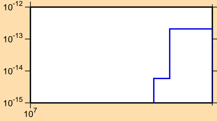
\sigma vs. E for ^{240}\text{Bk} (mt 34)
