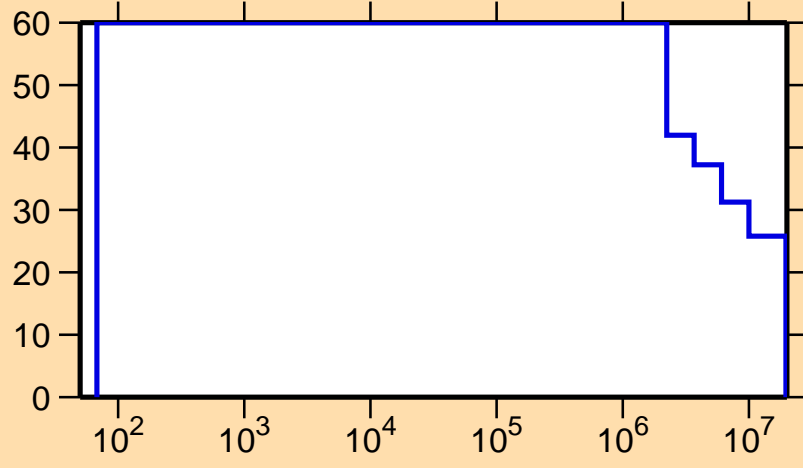
\Delta\sigma/\sigma vs. E for ^{240}\text{Bk}(n,p)
