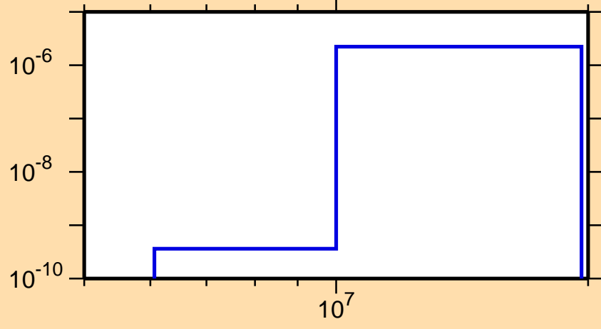
\sigma vs. E for ^{240}\text{Bk}(\text{mt } 45)
