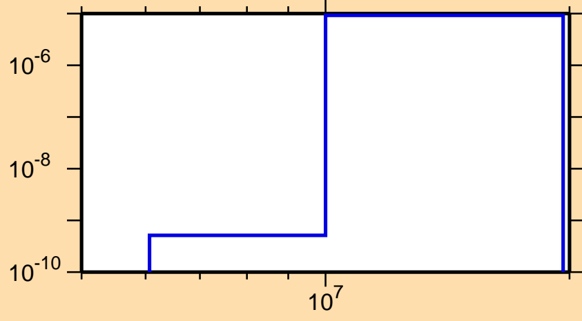
\sigma vs. E for ^{240}\text{Bk}(\text{mt117})
