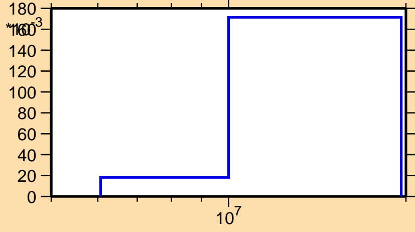
\sigma vs. E for ^{240}\text{Bk}(n,2n\alpha)
