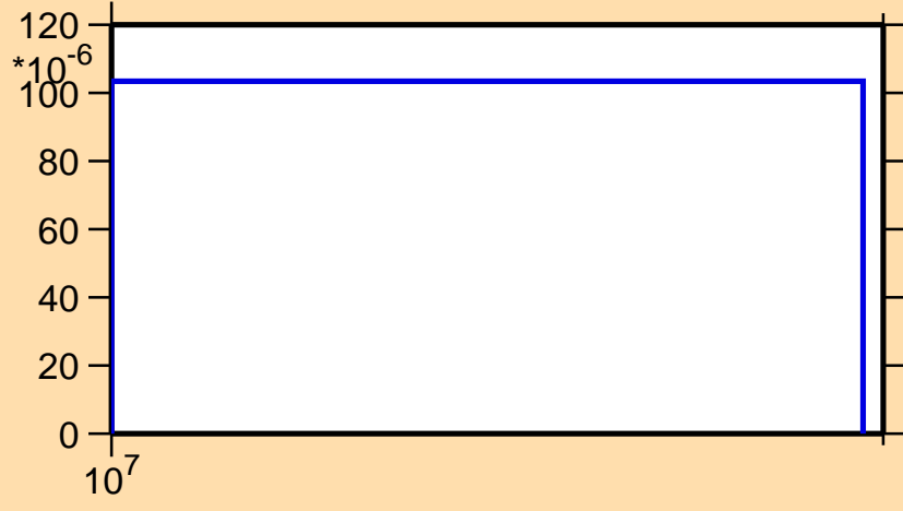
\sigma vs. E for ^{240}\text{Bk}(n,3n\alpha)
