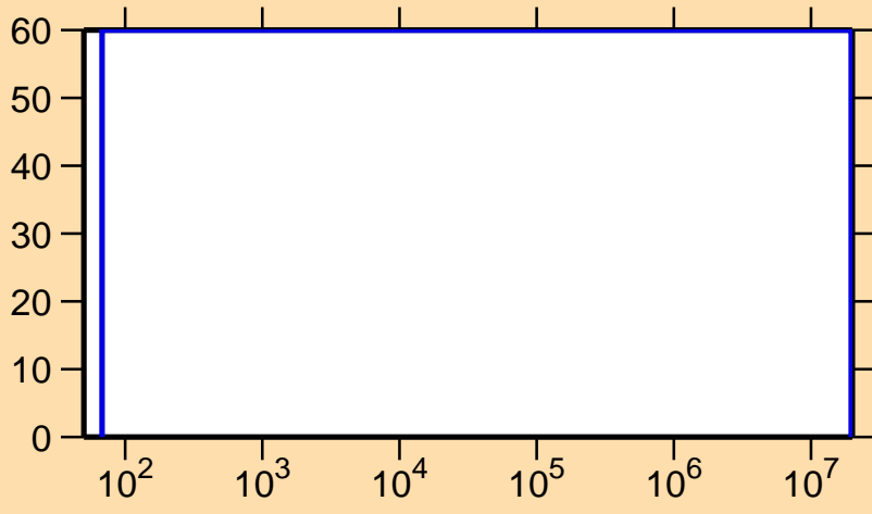
\Delta\sigma/\sigma vs. E for ^{240}\text{Bk}(n,\gamma)
