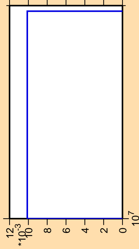
\Delta\sigma/\sigma vs. E for ^{240}\text{Bk} (mt 34)
