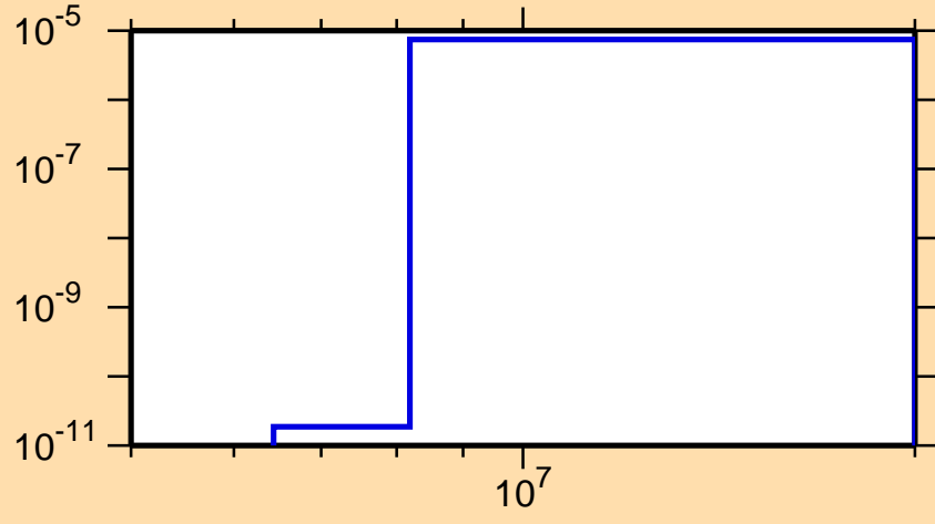
\sigma vs. E for ^{240}\text{Bk}(\text{mt117})
