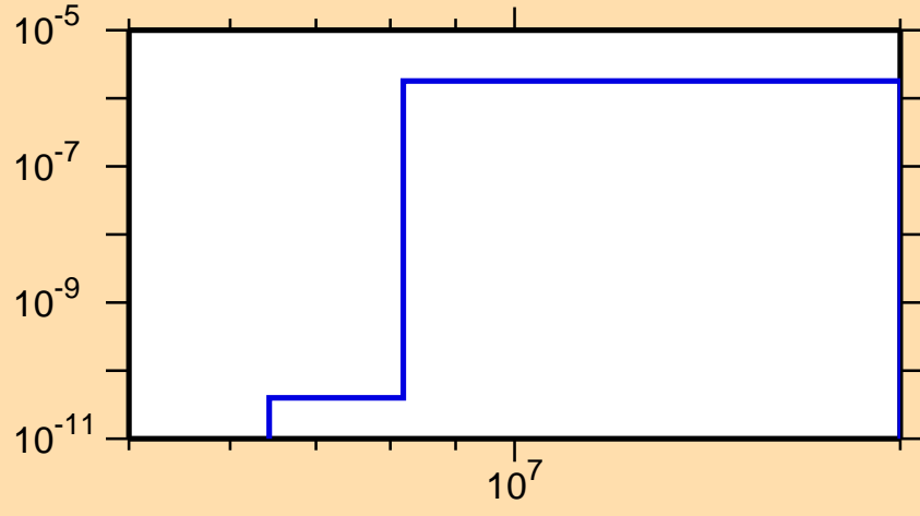
\sigma vs. E for ^{240}\text{Bk}(\text{mt } 45)
