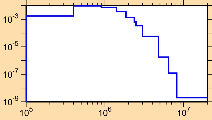
\sigma vs. E for ^{240}\text{Bk}(n,n_2)
