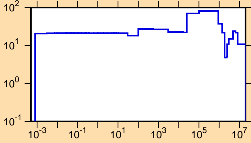
\Delta\sigma/\sigma vs. E for ^{240}\text{Bk}(n,el.)
