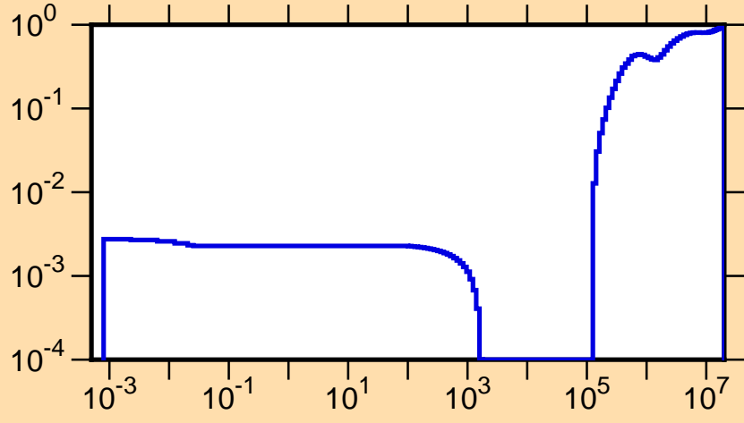
\mu vs. E for ^{242}\text{Bk}(\text{mt251})
