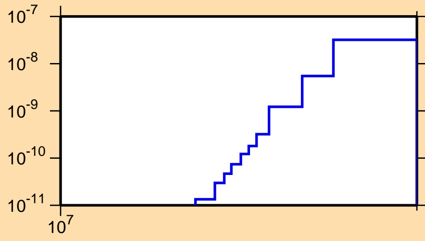
\sigma vs. E for ^{242}\text{Bk}(n,\text{He3})
