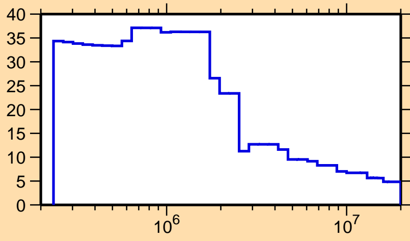
\Delta\sigma/\sigma vs. E for ^{242}\text{Bk}(n,\text{nonel.})
