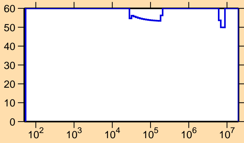
\Delta\sigma/\sigma vs. E for ^{242}\text{Bk}(n,\gamma)
