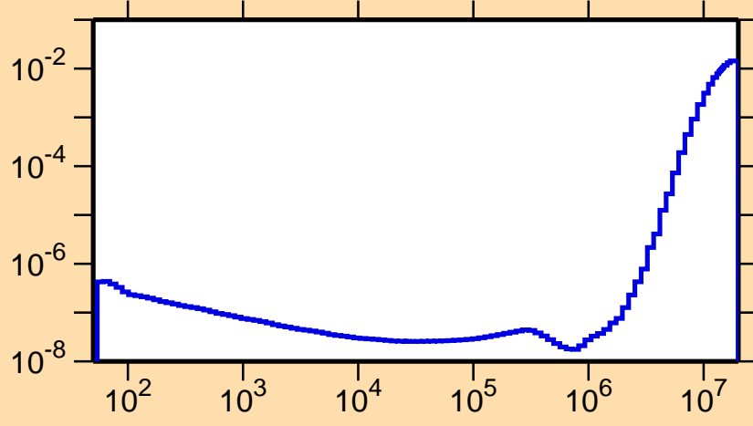
\sigma vs. E for ^{242}\text{Bk}(n,p)
