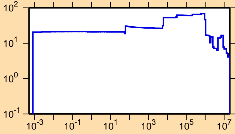
\Delta\sigma/\sigma vs. E for ^{242}\text{Bk}(n,el.)
