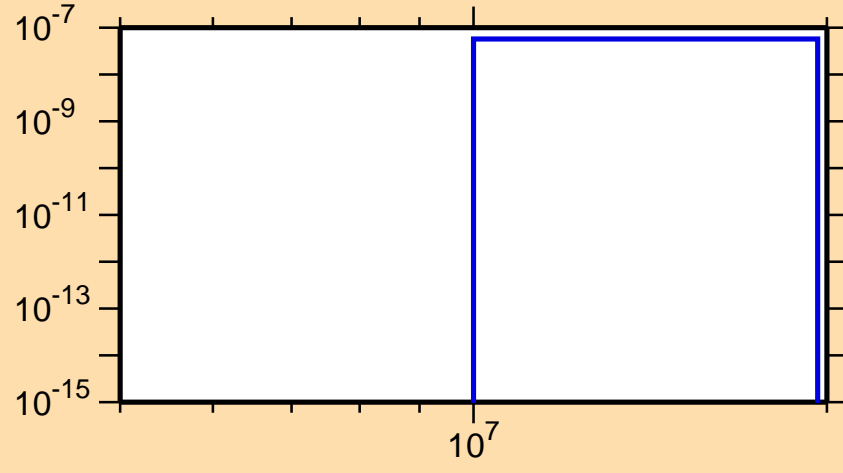
\sigma vs. E for ^{242}\text{Bk}(n,2np)
