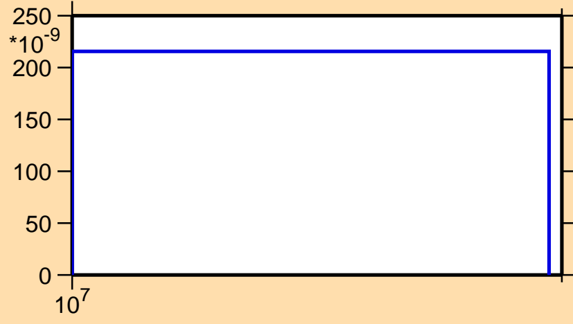
\sigma vs. E for ^{242}\text{Bk}(n,nd)
