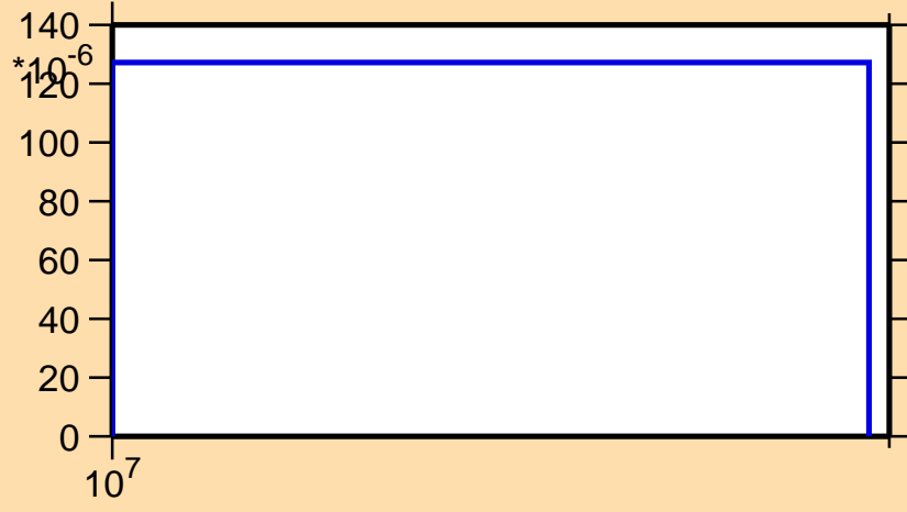
\sigma vs. E for ^{242}\text{Bk}(n,3n\alpha)
