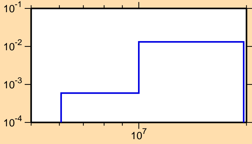
\sigma vs. E for ^{242}\text{Bk}(n,2n\alpha)
