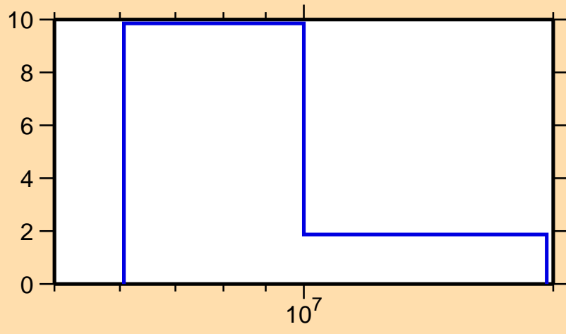
\Delta\sigma/\sigma vs. E for ^{242}\text{Bk}(n,\text{tot.})
