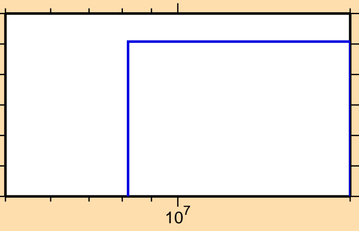
\sigma vs. E for ^{242}\text{Bk}(n,nt)
