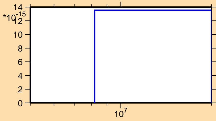
\sigma vs. E for ^{242}\text{Bk} (mt 34)
