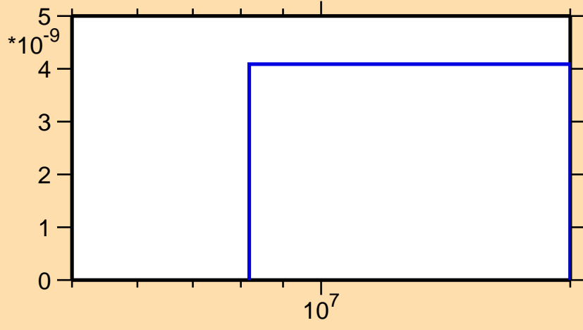
\sigma vs. E for ^{242}\text{Bk} (mt 45)
