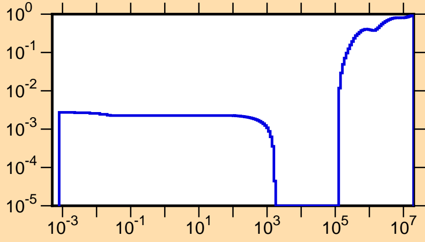
\mu vs. E for ^{243}\text{Bk}(\text{mt251})
