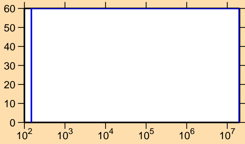
\Delta\sigma/\sigma vs. E for ^{243}\text{Bk}(n,\gamma)
