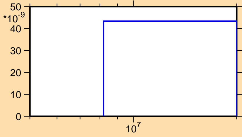
\sigma vs. E for ^{243}\text{Bk}(n,nd)
