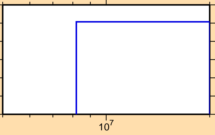
\sigma vs. E for ^{243}\text{Bk}(n,nt)
