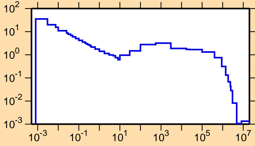
\sigma vs. E for ^{243}\text{Bk}(n,\gamma)
