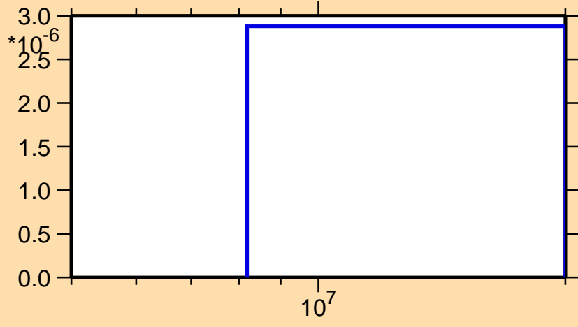
\sigma vs. E for ^{243}\text{Bk} (mt 45)
