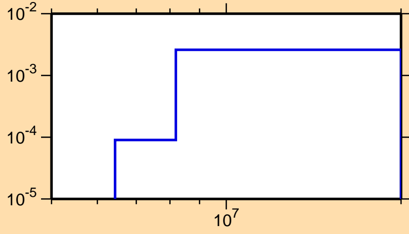
\sigma vs. E for ^{243}\text{Bk}(n,2n\alpha)
