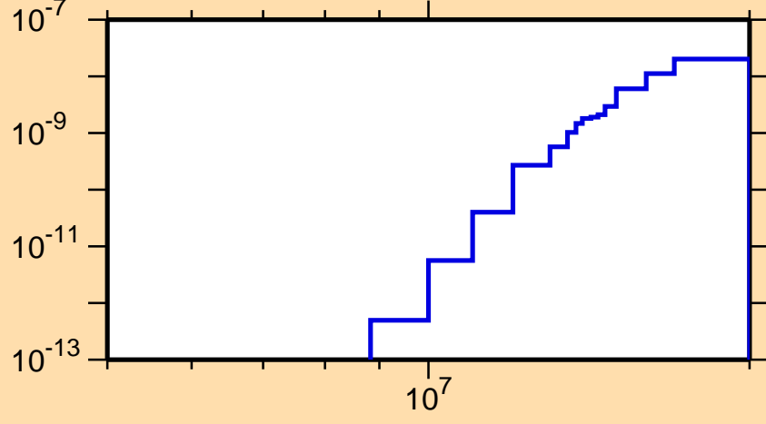
\sigma vs. E for ^{244}\text{Bk}(\text{mt117})
