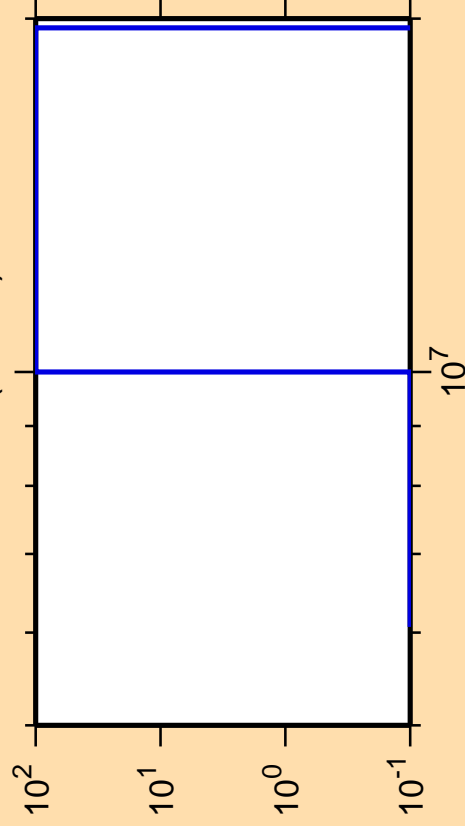
\Delta\sigma/\sigma vs. E for ^{244}\text{Bk}(\text{mt } 45)
