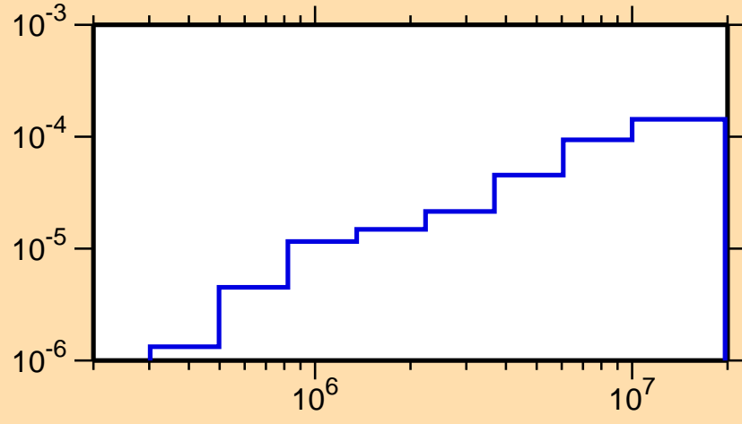
\sigma vs. E for ^{244}\text{Bk}(n,n\alpha)
