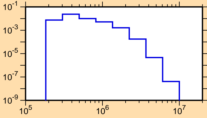
\sigma vs. E for ^{244}\text{Bk}(n,n_3)
