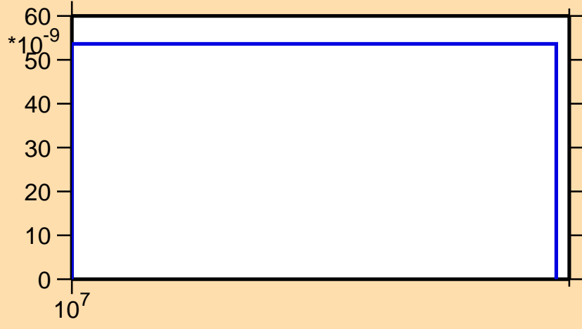
\sigma vs. E for ^{244}\text{Bk}(n,2np)
