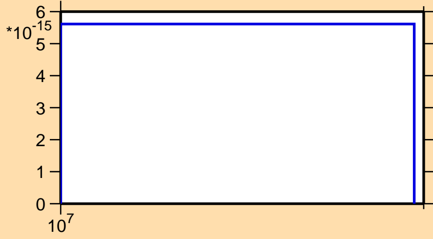
\sigma vs. E for ^{244}\text{Bk} (mt 34)
