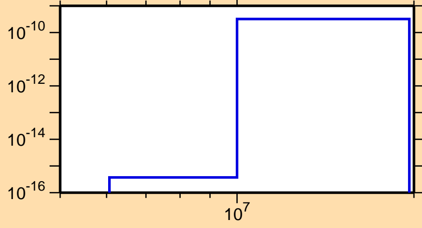
\sigma vs. E for ^{244}\text{Bk}(\text{mt } 45)
