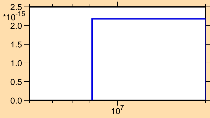
\sigma vs. E for ^{244}\text{Bk}(\text{mt } 11)
