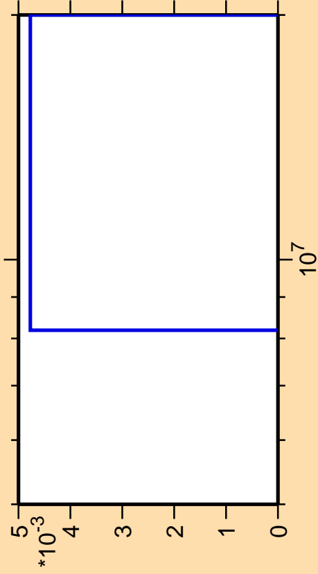
\Delta\sigma/\sigma vs. E for ^{244}\text{Bk}(\text{mt } 34)
