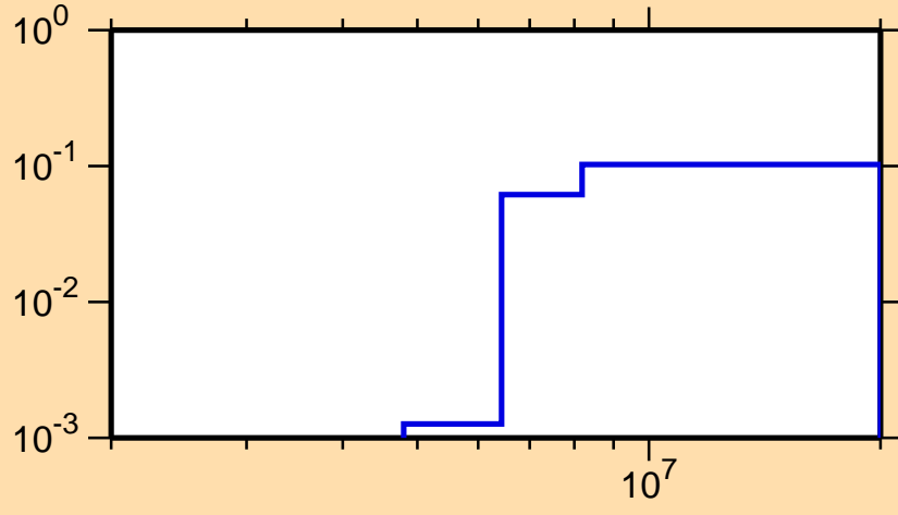
\sigma vs. E for ^{244}\text{Bk}(n,2n)
