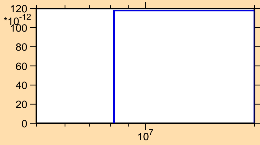
\sigma vs. E for ^{244}\text{Bk}(n,\text{He3})
