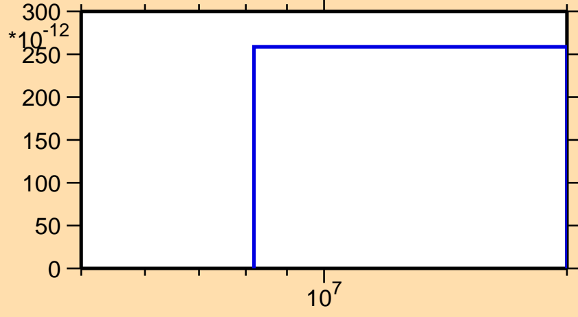
\sigma vs. E for ^{244}\text{Bk} (mt 45)
