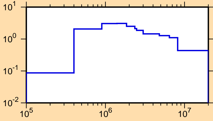
\sigma vs. E for ^{244}\text{Bk}(n,\text{inel.})
