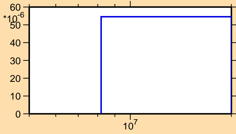
\sigma vs. E for ^{244}\text{Bk}(n,3n\alpha)
