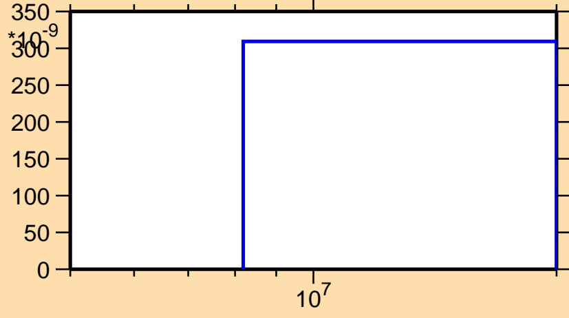
\sigma vs. E for ^{244}\text{Bk}(n,nd)
