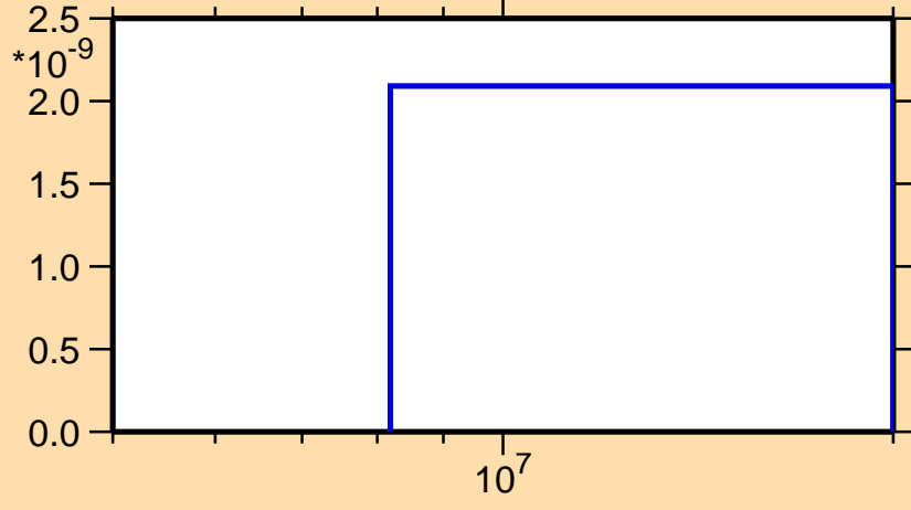
\sigma vs. E for ^{244}\text{Bk}(\text{mt117})
