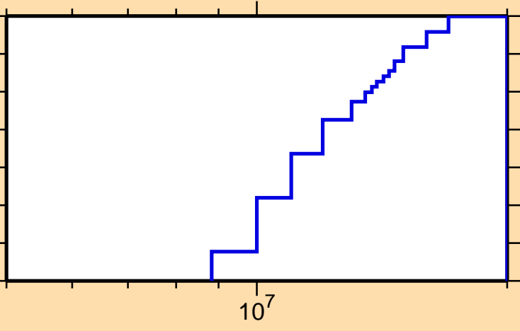
\sigma vs. E for ^{245}\text{Bk}(\text{mt117})
