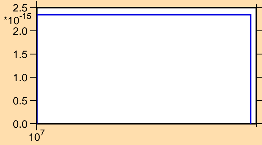
\sigma vs. E for ^{245}\text{Bk} (mt 11)
