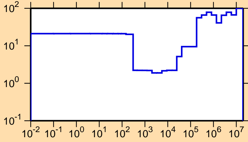
\Delta\sigma/\sigma vs. E for ^{245}\text{Bk}(n,el.)
