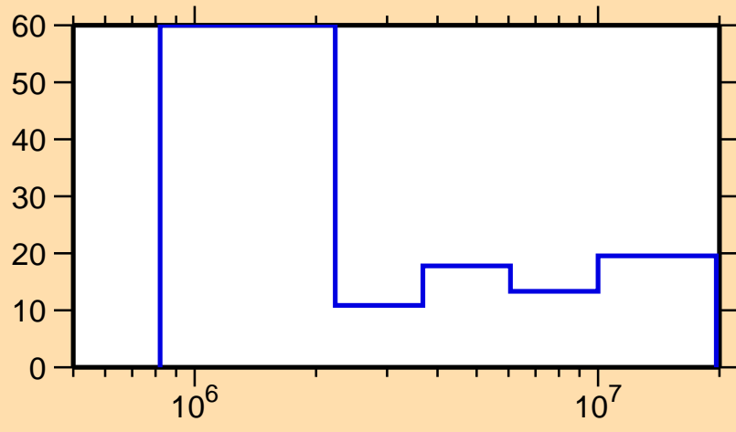
\Delta\sigma/\sigma vs. E for ^{245}\text{Bk}(n,f)
