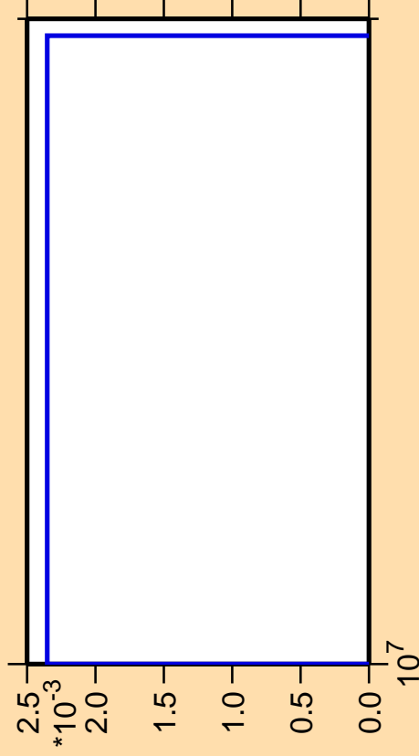
\Delta\sigma/\sigma vs. E for ^{245}\text{Bk} (mt 11)
