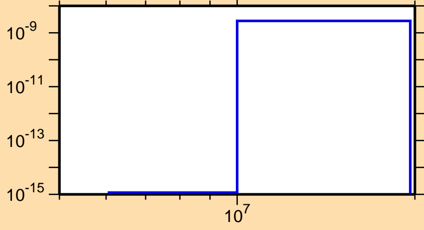
\sigma vs. E for ^{245}\text{Bk}(\text{mt } 45)
