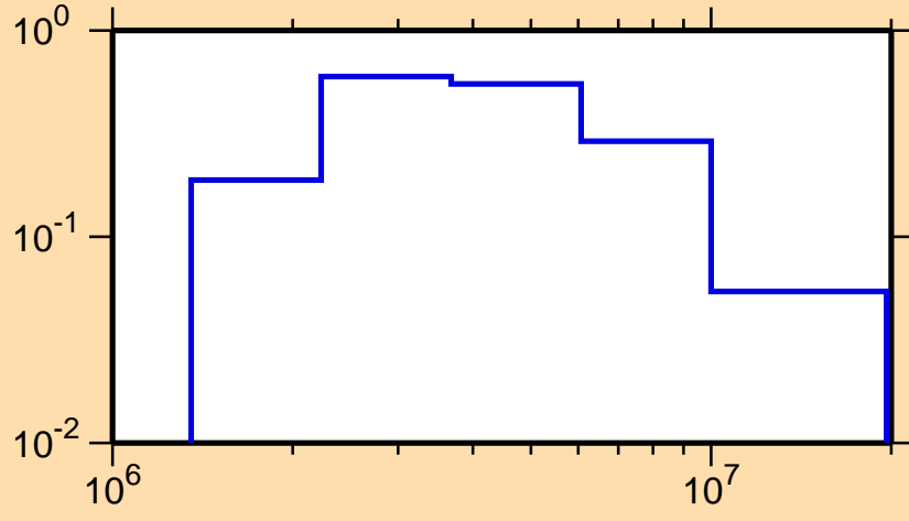
\sigma vs. E for ^{245}\text{Bk}(n,n\text{cont.})
