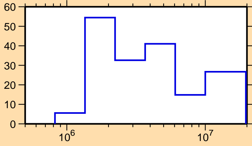
\Delta\sigma/\sigma vs. E for ^{245}\text{Bk}(n,p)
