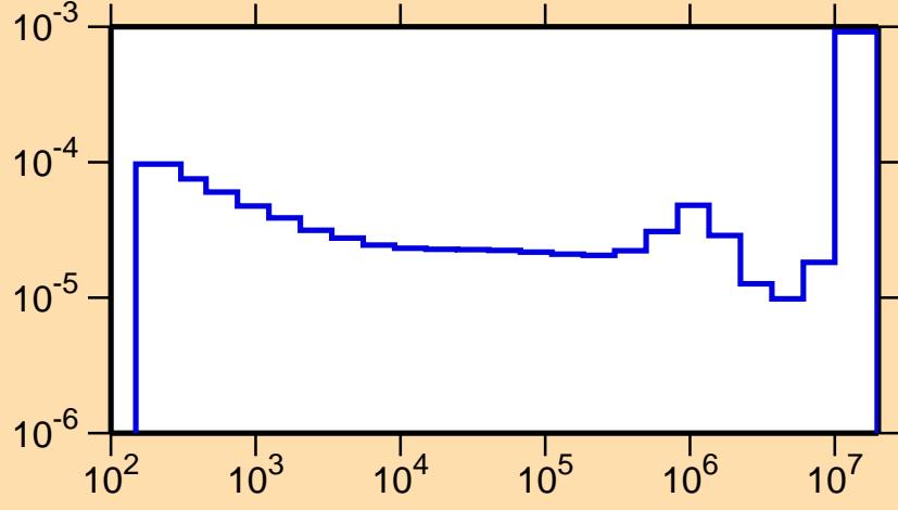
\sigma vs. E for ^{245}\text{Bk}(n,\alpha)
