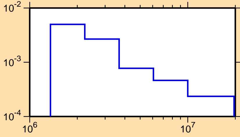
\sigma vs. E for ^{245}\text{Bk}(n,n_1)
