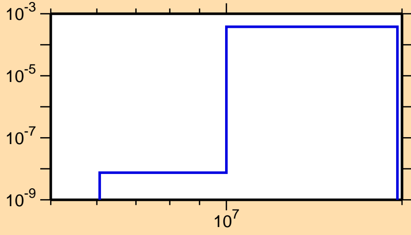
\sigma vs. E for ^{245}\text{Bk}(n,d)
