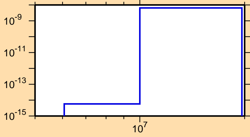
\sigma vs. E for ^{245}\text{Bk}(\text{mt117})
