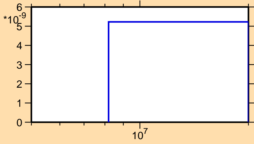
\sigma vs. E for ^{245}\text{Bk}(\text{mt117})
