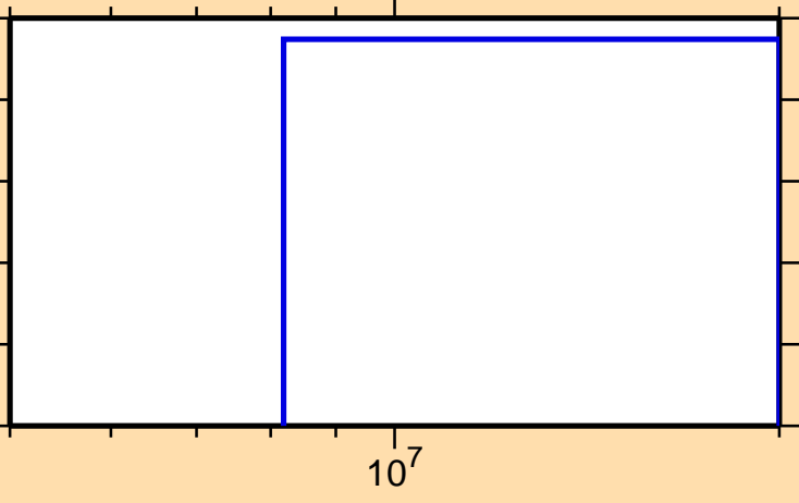
\sigma vs. E for ^{245}\text{Bk}(n,2np)
