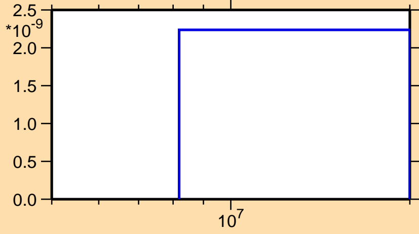
\sigma vs. E for ^{245}\text{Bk} (mt 45)
