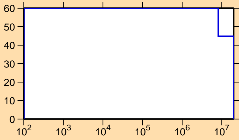
\Delta\sigma/\sigma vs. E for ^{245}\text{Bk}(n,\gamma)
