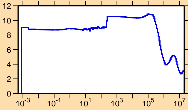
\sigma vs. E for ^{246}\text{Bk}(n,\text{el.})
