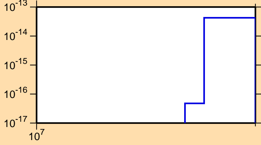
\sigma vs. E for ^{246}\text{Bk} (mt 34)
