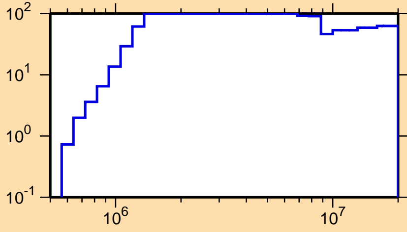
\Delta\sigma/\sigma vs. E for ^{246}\text{Bk}(n,p)
