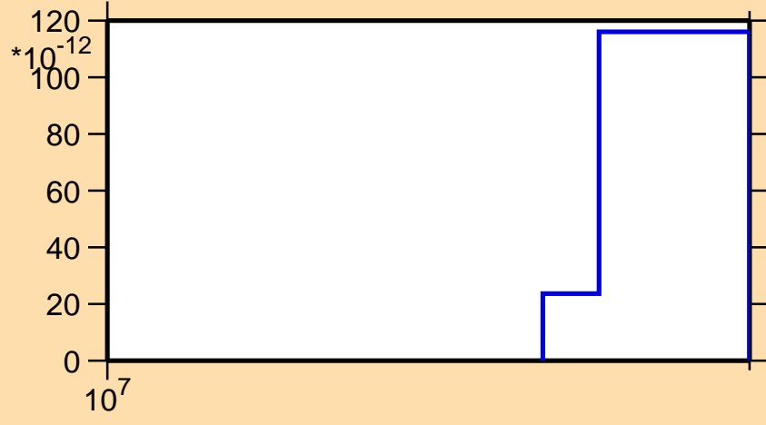
\sigma vs. E for ^{246}\text{Bk} (mt 45)
