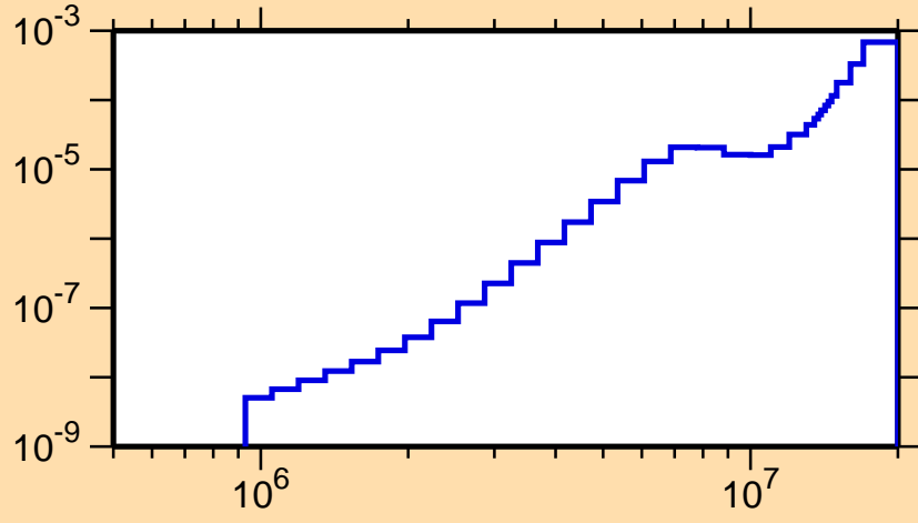
\sigma vs. E for ^{246}\text{Bk}(n,n\alpha)
