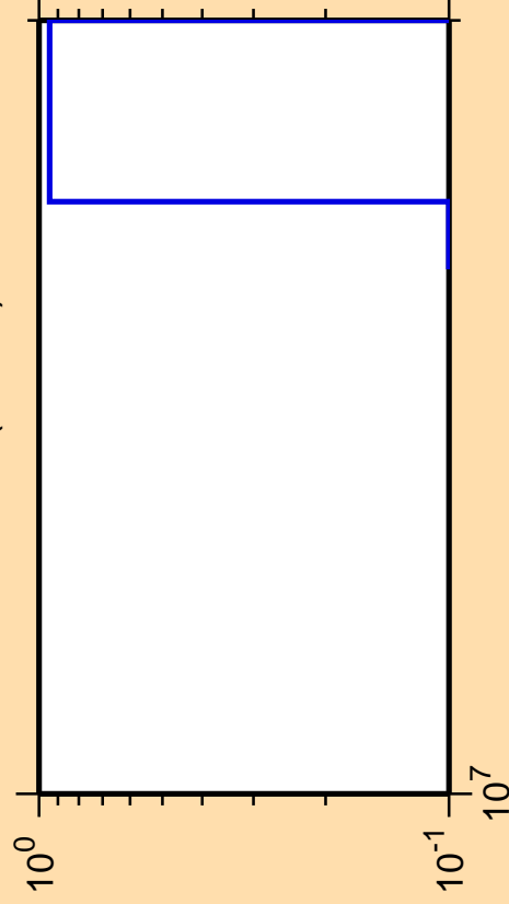
\Delta\sigma/\sigma vs. E for ^{246}\text{Bk} (mt 11)
