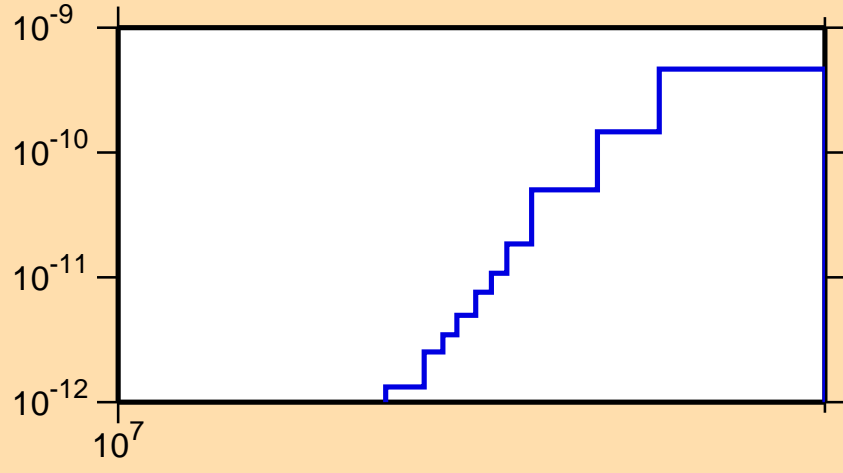
\sigma vs. E for ^{246}\text{Bk}(\text{mt117})
