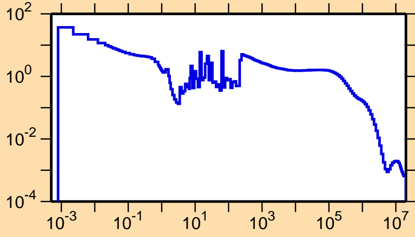
\sigma vs. E for ^{246}\text{Bk}(n,\gamma)
