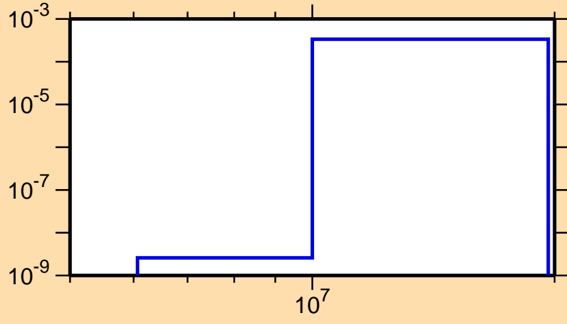
\sigma vs. E for ^{246}\text{Bk}(n,d)
