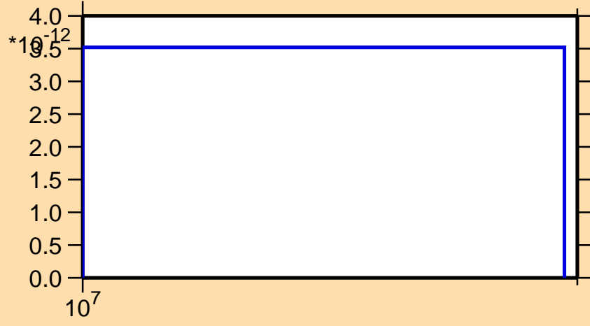
\sigma vs. E for ^{246}\text{Bk}(\text{mt } 45)
