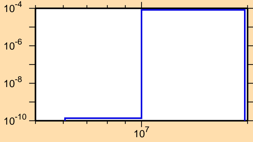
\sigma vs. E for ^{246}\text{Bk}(n,t)
