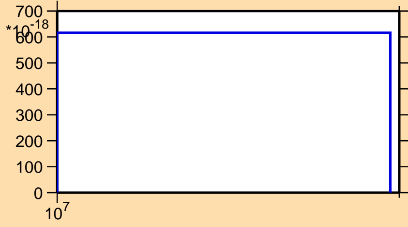
\sigma vs. E for ^{246}\text{Bk} (mt 11)
