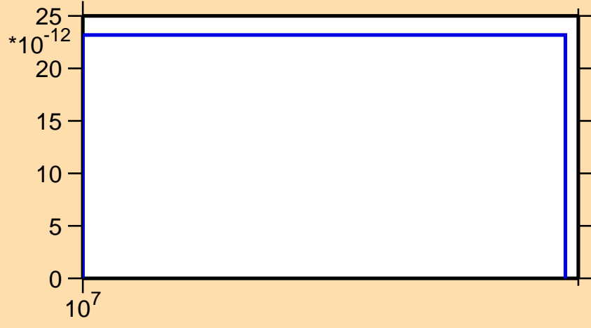
\sigma vs. E for ^{246}\text{Bk}(\text{mt117})
