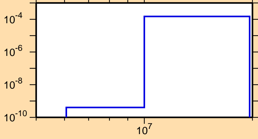
\sigma vs. E for ^{246}\text{Bk}(n,np)
