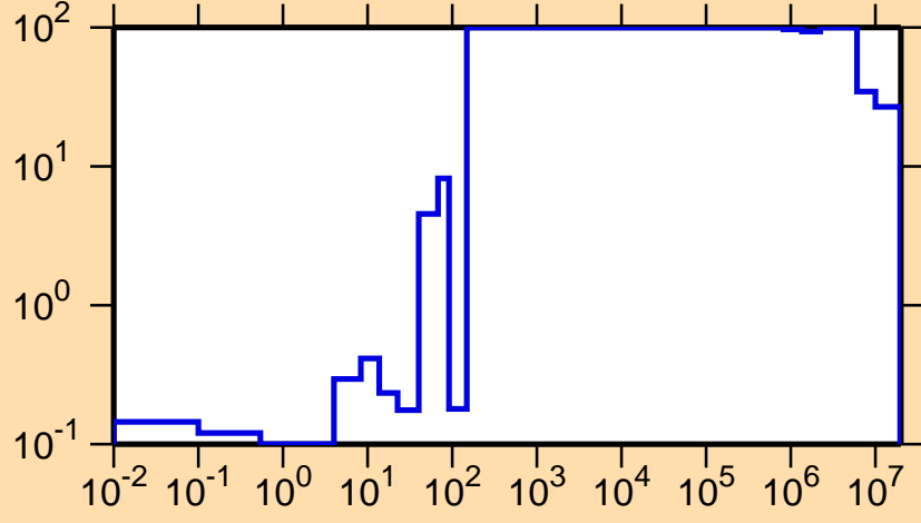
\Delta\sigma/\sigma vs. E for ^{246}\text{Bk}(n,f)
