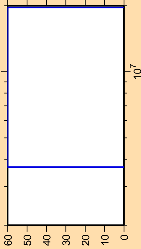
\Delta\sigma/\sigma vs. E for ^{246}\text{Bk}(n,n\text{cont.})
