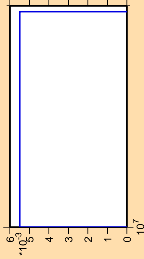
\Delta\sigma/\sigma vs. E for ^{246}\text{Bk} (mt 11)
