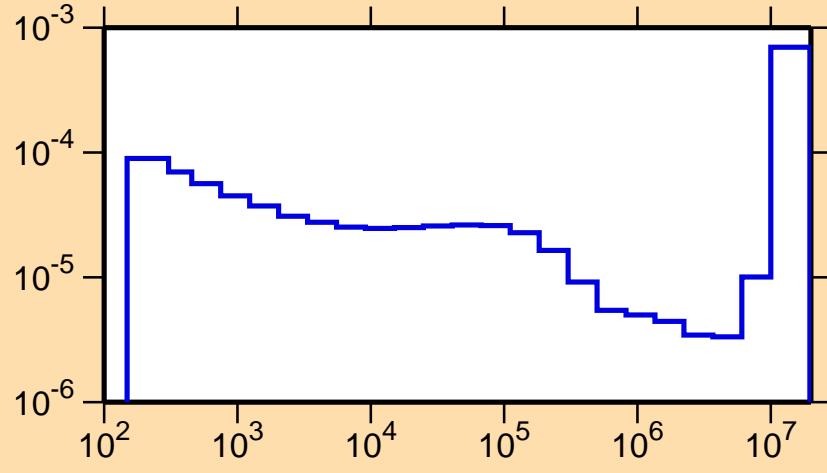
\sigma vs. E for ^{246}\text{Bk}(n,\alpha)
