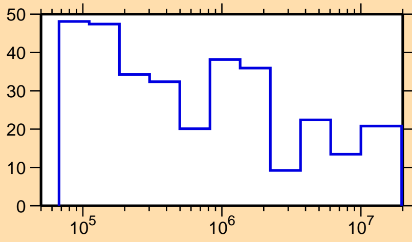
\Delta\sigma/\sigma vs. E for ^{246}\text{Bk}(n,\text{el.})
