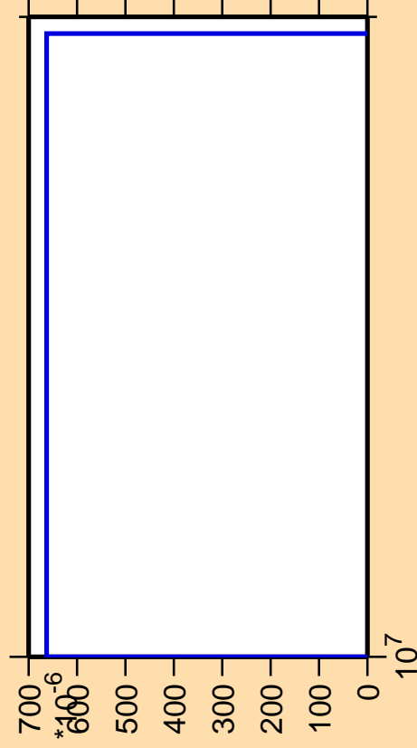
\Delta\sigma/\sigma vs. E for ^{246}\text{Bk}(\text{mt } 34)
