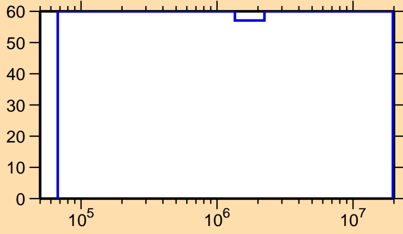
\Delta\sigma/\sigma vs. E for ^{246}\text{Bk}(n,n\text{cont.})
