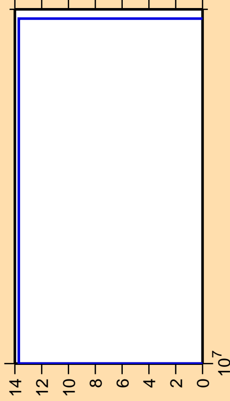
\Delta\sigma/\sigma vs. E for ^{246}\text{Bk}(\text{mt } 45)
