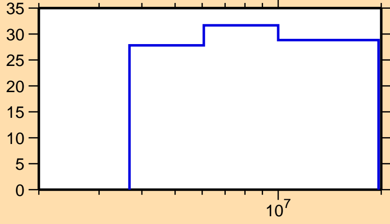
\Delta\sigma/\sigma vs. E for ^{246}\text{Bk}(n,\text{nonel.})
