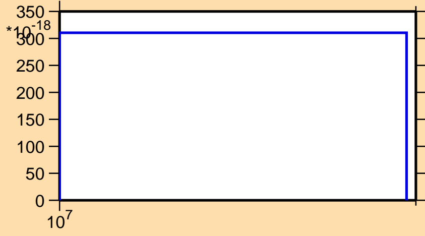
\sigma vs. E for ^{246}\text{Bk}(\text{mt } 34)
