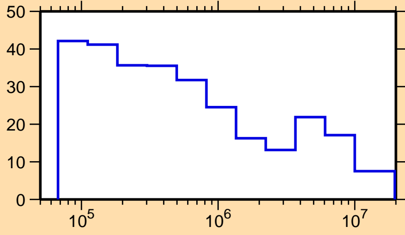
\Delta\sigma/\sigma vs. E for ^{246}\text{Bk}(n, tot.)
