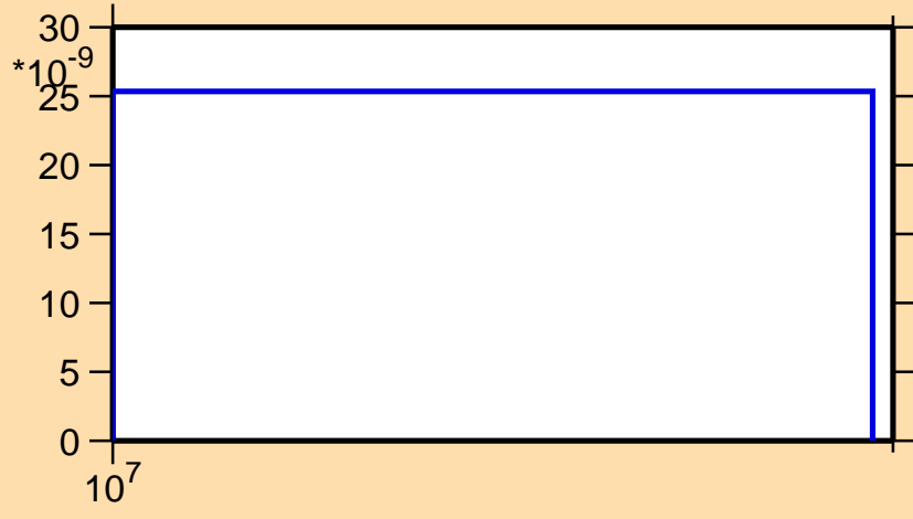
\sigma vs. E for ^{246}\text{Bk}(n,nt)
