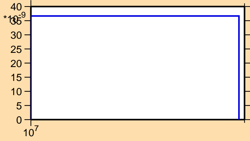
\sigma vs. E for ^{246}\text{Bk}(n,2np)
