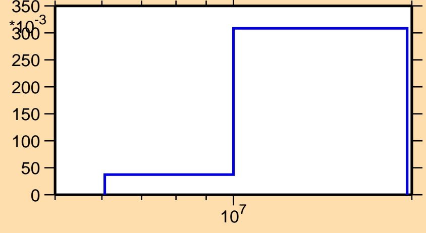
\sigma vs. E for ^{246}\text{Bk}(n,2n\alpha)
