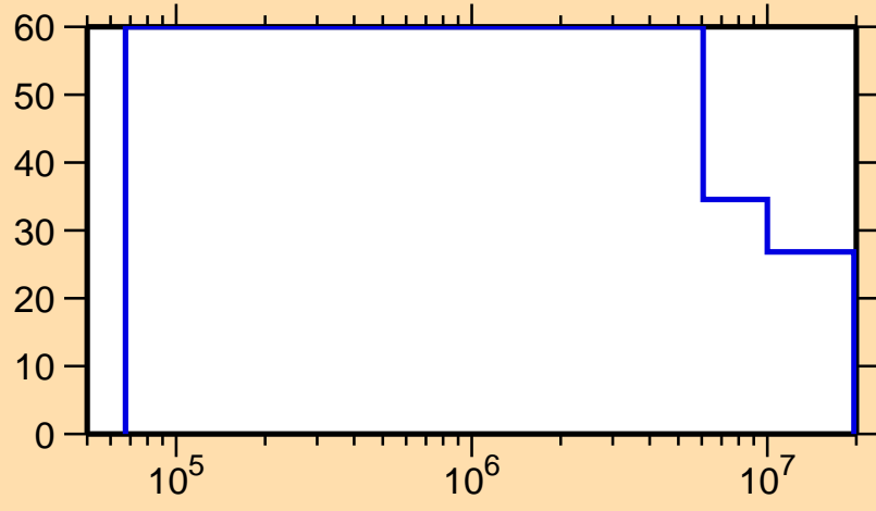
\Delta\sigma/\sigma vs. E for ^{246}\text{Bk}(n,f)
