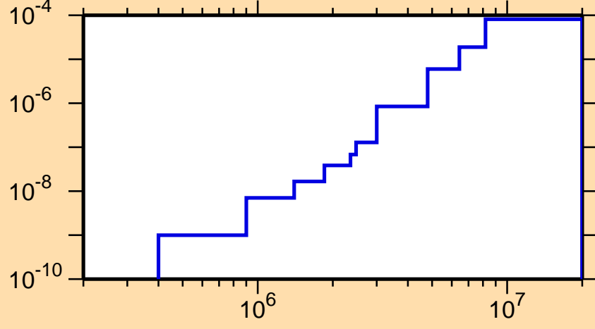
\sigma vs. E for ^{246}\text{Bk}(n,n\alpha)
