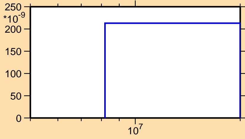
\sigma vs. E for ^{246}\text{Bk}(n,nd)
