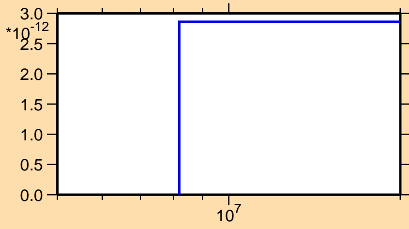
\sigma vs. E for ^{246}\text{Bk} (mt 45)
