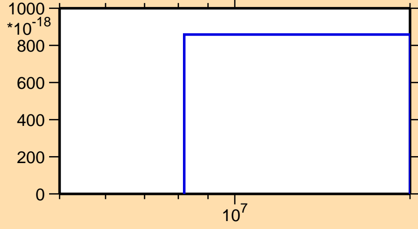
\sigma vs. E for ^{246}\text{Bk}(\text{mt } 11)
