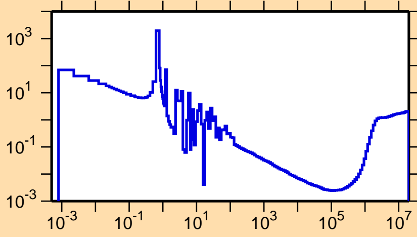
\sigma vs. E for ^{247}\text{Bk}(n,f)
