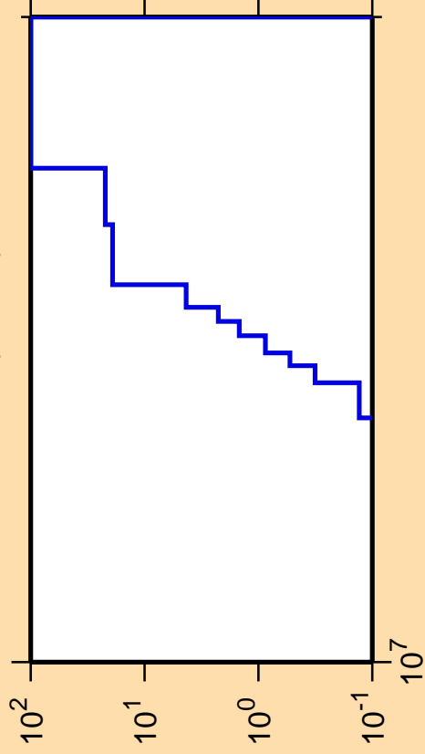
\Delta\sigma/\sigma vs. E for ^{247}\text{Bk}(\text{mt } 45)
