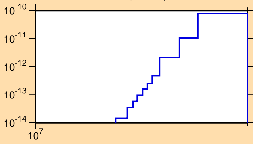
\sigma vs. E for ^{247}\text{Bk}(\text{mt } 45)
