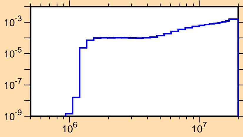
\sigma vs. E for ^{247}\text{Bk}(n,n\alpha)
