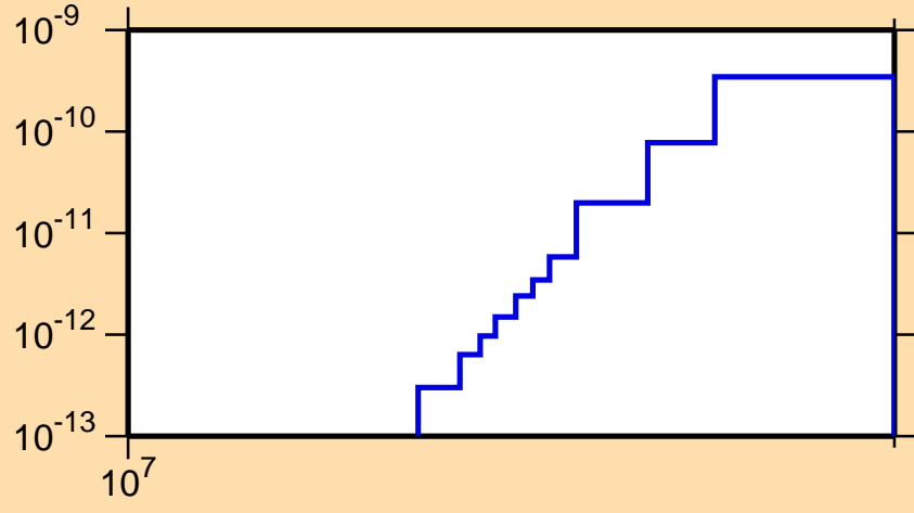
\sigma vs. E for ^{247}\text{Bk}(\text{mt117})
