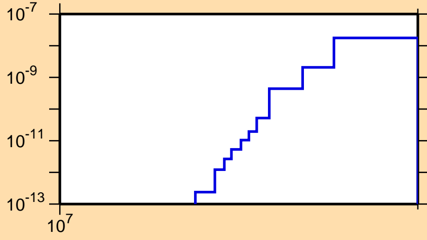
\sigma vs. E for ^{248}\text{Bk}(\text{mt } 45)
