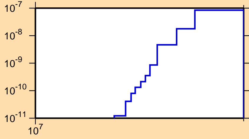
\sigma vs. E for ^{248}\text{Bk}(\text{mt117})
