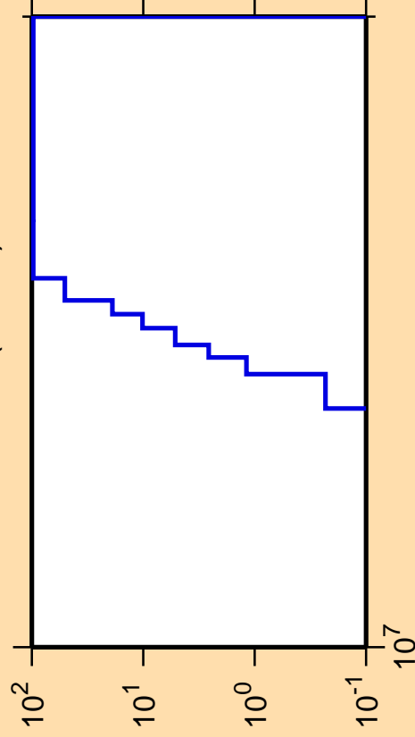
\Delta\sigma/\sigma vs. E for ^{248}\text{Bk}(\text{mt } 45)
