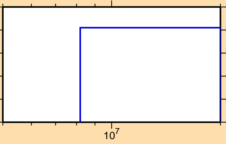
\sigma vs. E for ^{248}\text{Bk}(\text{mt117})
