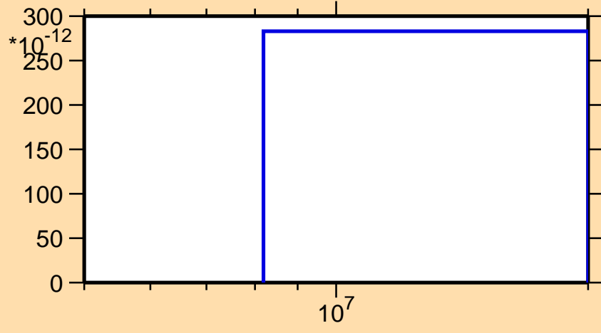
\sigma vs. E for ^{248}\text{Bk} (mt 45)
