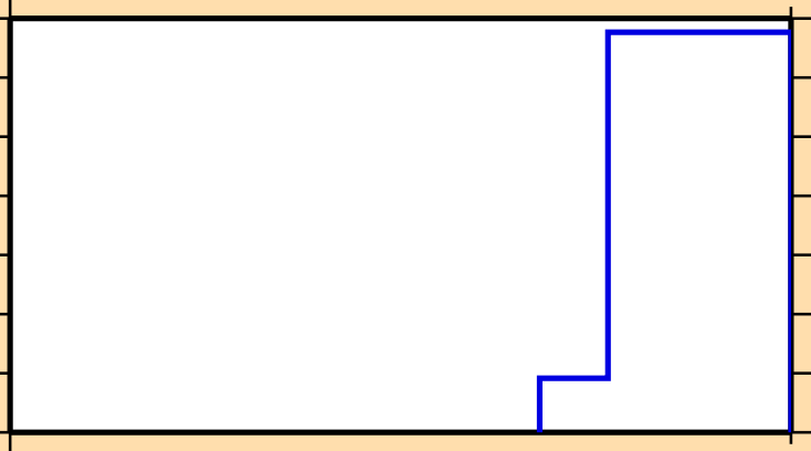
\sigma vs. E for ^{248}\text{Bk} (mt 11)
