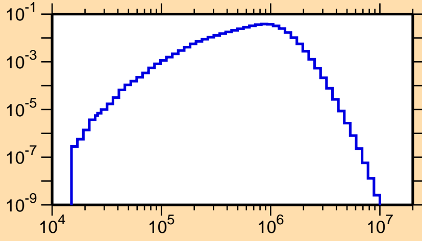
\sigma vs. E for ^{248}\text{Bk}(n,n_3)
