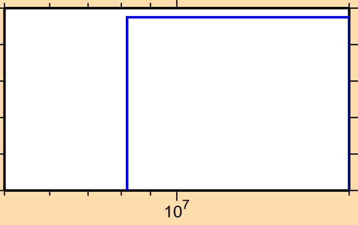
\sigma vs. E for ^{248}\text{Bk} (mt 11)
