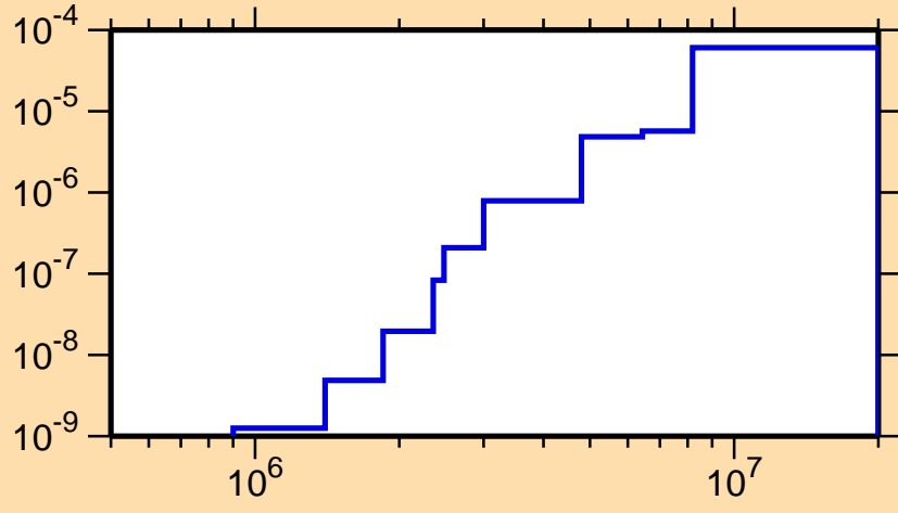
\sigma vs. E for ^{248}\text{Bk}(n,n\alpha)
