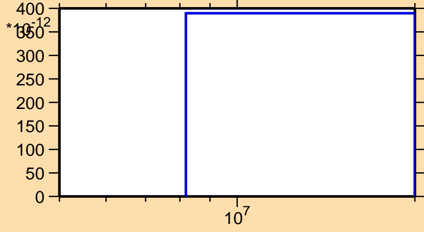
\sigma vs. E for ^{248}\text{Bk}(n,p\alpha)
