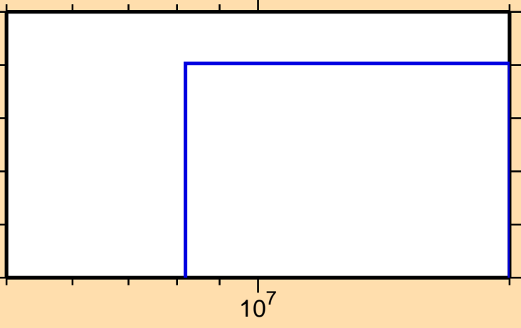
\sigma vs. E for ^{248}\text{Bk} (mt 45)
