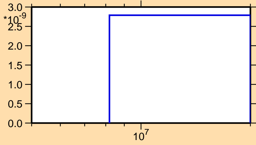
\sigma vs. E for ^{248}\text{Bk}(\text{mt117})
