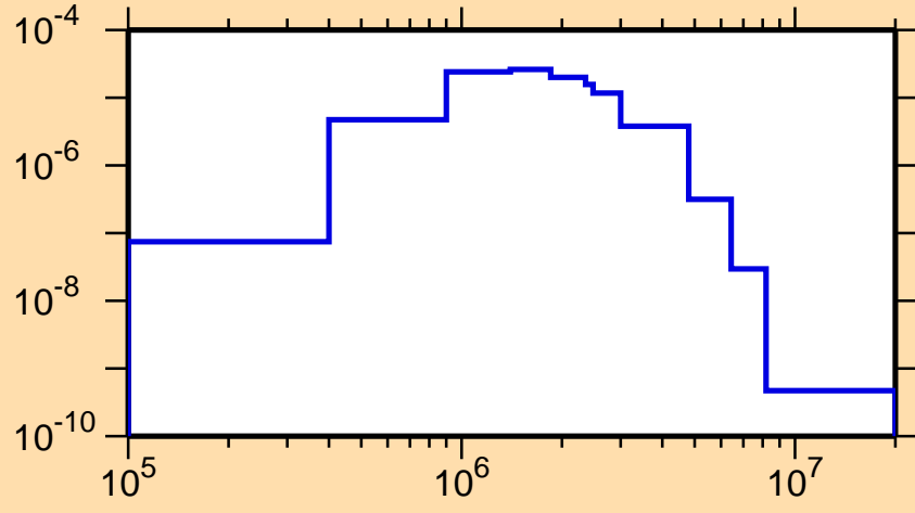
\sigma vs. E for ^{248}\text{Bk}(n,n_2)
