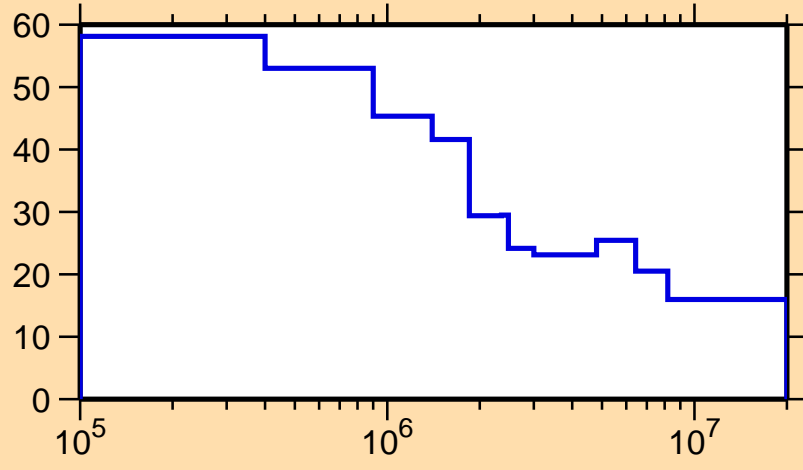
\Delta\sigma/\sigma vs. E for ^{248}\text{Bk}(n,n\text{onel.})
