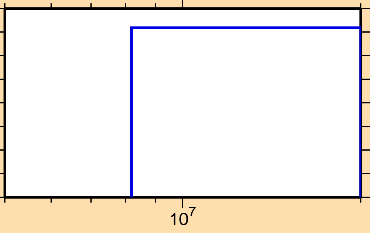
\sigma vs. E for ^{248}\text{Bk}(n,nt)
