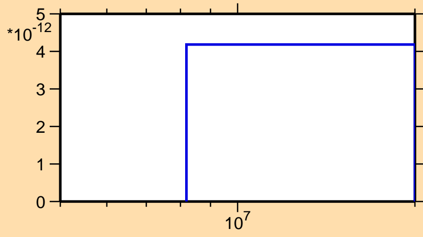
\sigma vs. E for ^{249}\text{Bk}(n,p\alpha)
