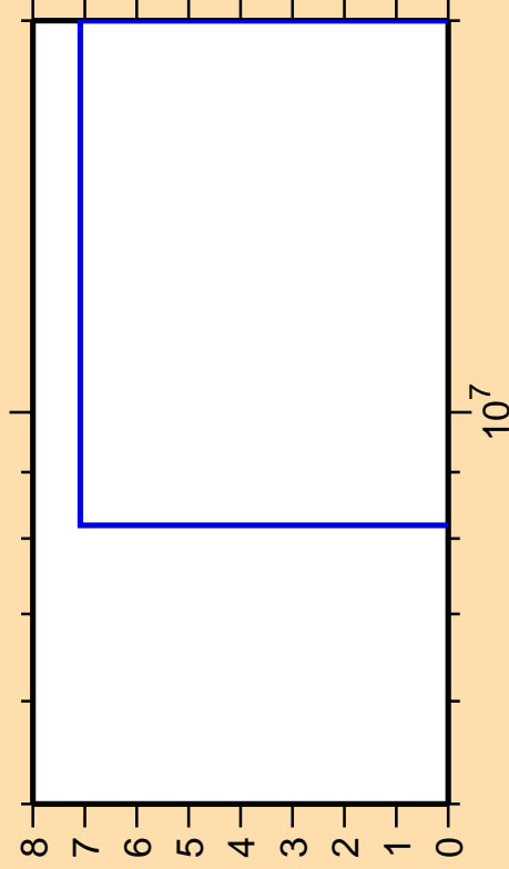
\Delta\sigma/\sigma vs. E for ^{249}\text{Bk}(n,t)
