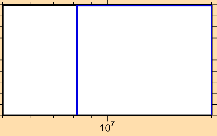
\sigma vs. E for ^{249}\text{Bk}(n,3n\alpha)
