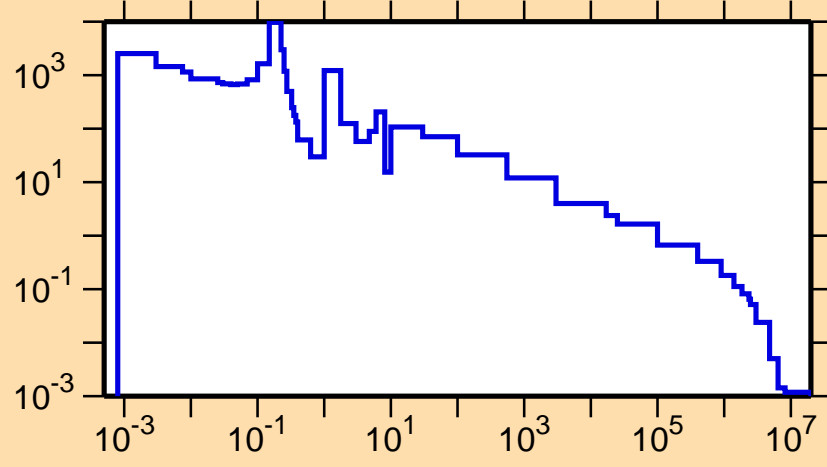
\sigma vs. E for ^{249}\text{Bk}(n,\gamma)
