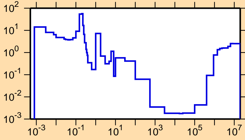
\sigma vs. E for ^{249}\text{Bk}(n,f)
