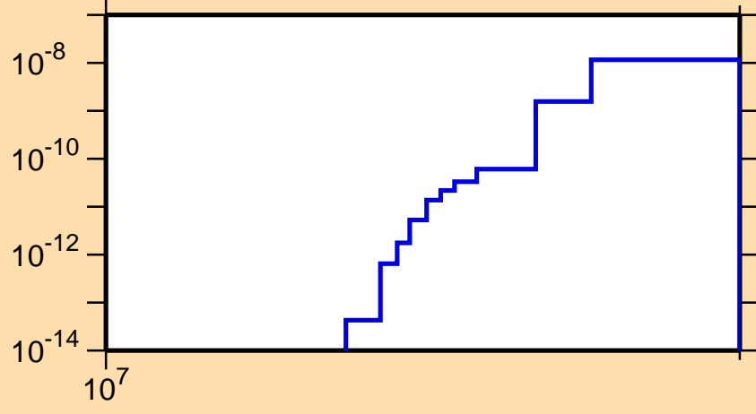
\sigma vs. E for ^{250}\text{Bk}(\text{mt } 45)
