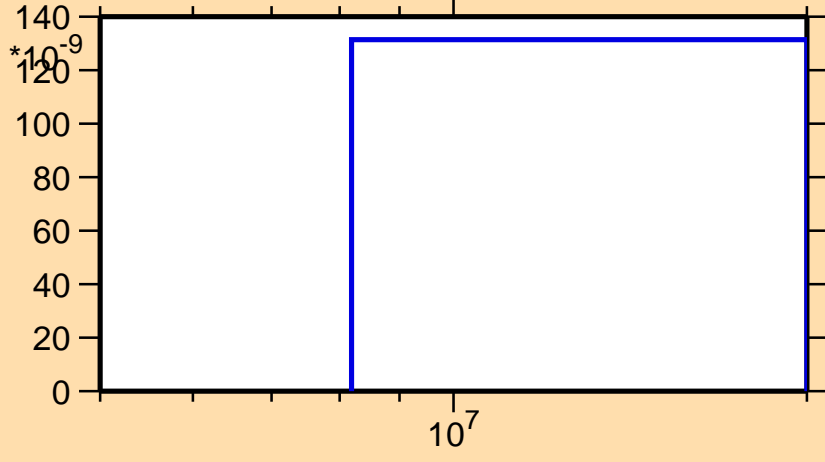
\sigma vs. E for ^{250}\text{Bk}(n,nt)
