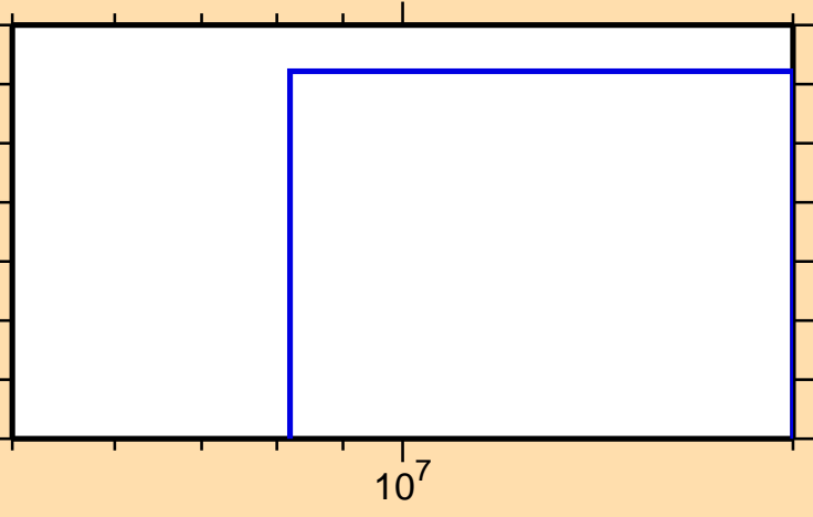
\sigma vs. E for ^{250}\text{Bk}(n,nd)
