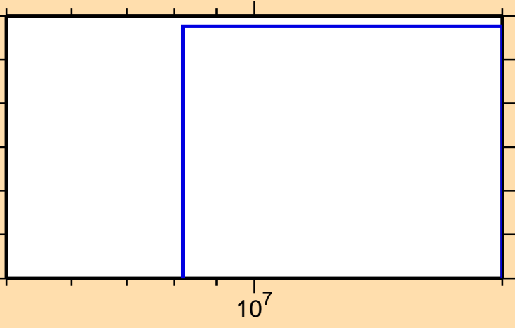
\sigma vs. E for ^{250}\text{Bk}(n,2np)
