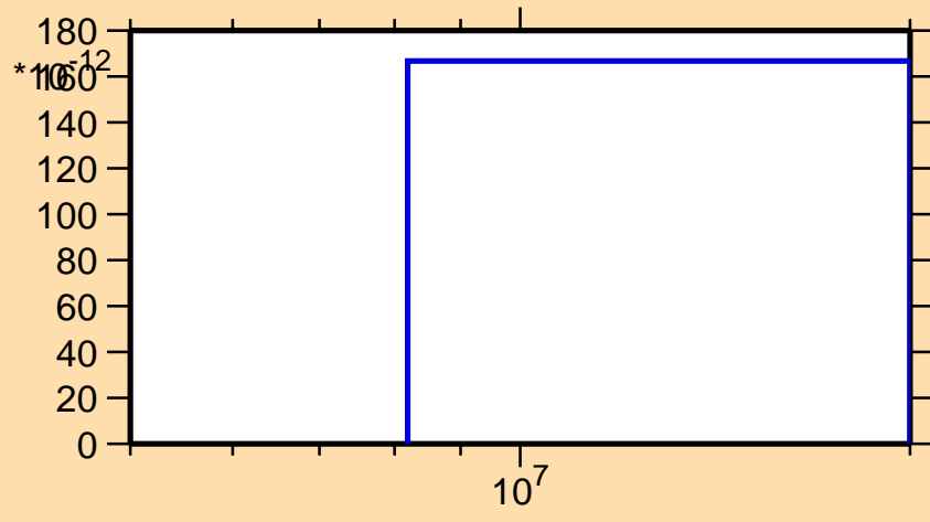
\sigma vs. E for ^{250}\text{Bk}(\text{mt } 45)
