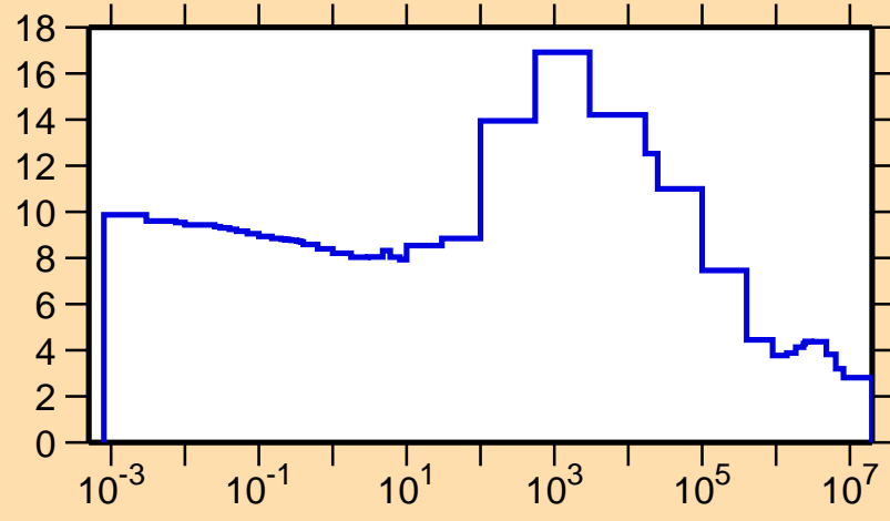
\sigma vs. E for ^{250}\text{Bk}(n,el.)
