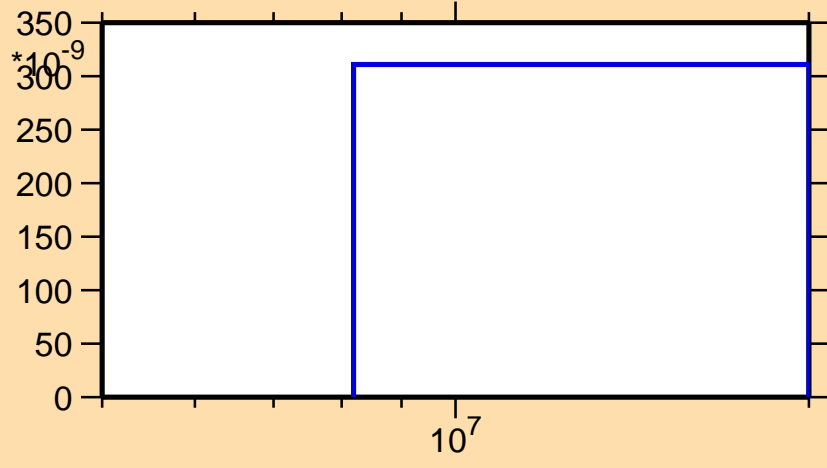
\sigma vs. E for ^{250}\text{Bk}(n,nd)
