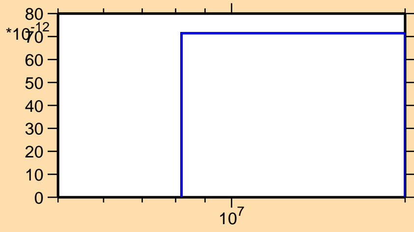
\sigma vs. E for ^{250}\text{Bk}(n,p\alpha)
