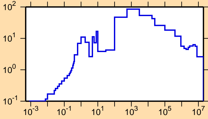
\Delta\sigma/\sigma vs. E for ^{250}\text{Bk}(n,tot.)
