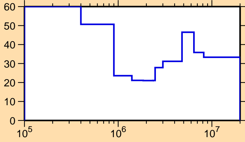
\Delta\sigma/\sigma vs. E for ^{250}\text{Bk}(n,n\text{cont.})
