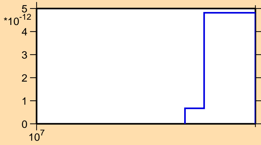
\sigma vs. E for ^{251}\text{Bk} (mt 45)
