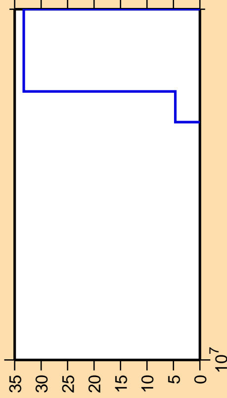
\Delta\sigma/\sigma vs. E for ^{251}\text{Bk} (mt 45)
