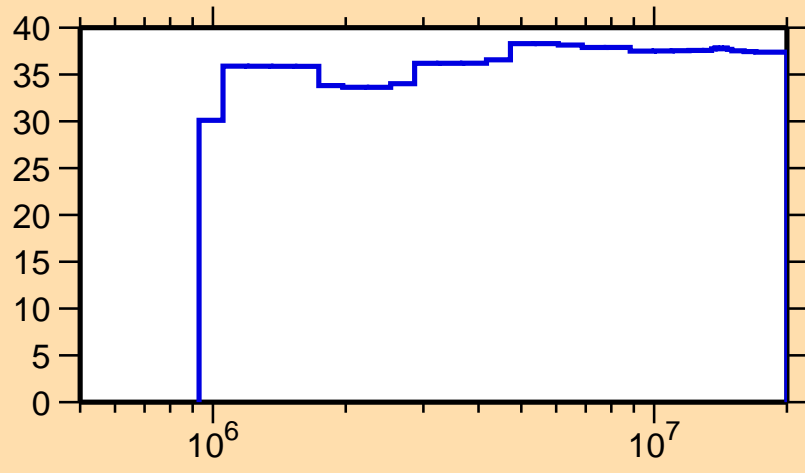
\Delta\sigma/\sigma vs. E for ^{251}\text{Bk}(n,n_1)
