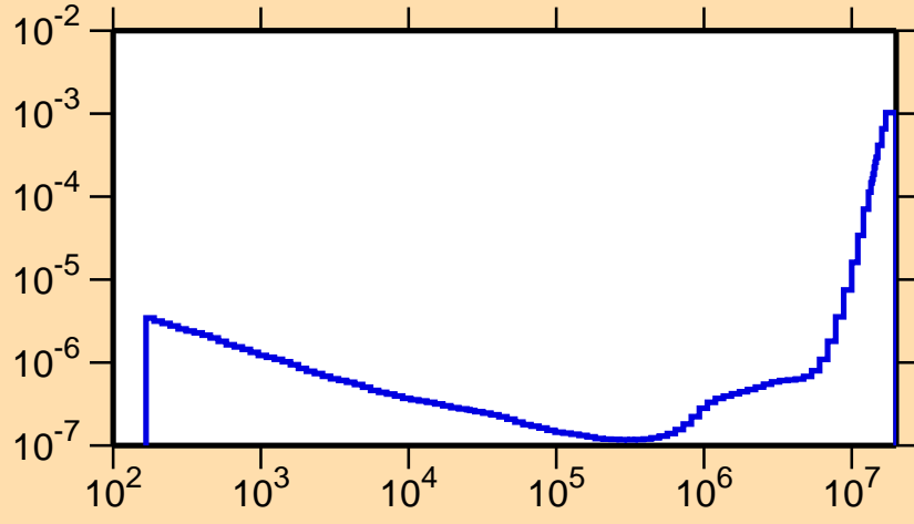
\sigma vs. E for ^{251}\text{Bk}(n,\alpha)
