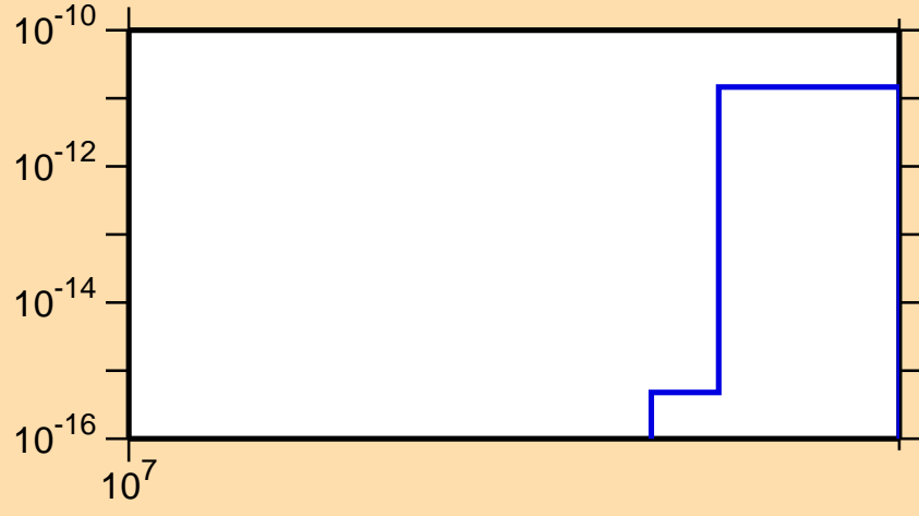
\sigma vs. E for ^{251}\text{Bk} (mt 11)
