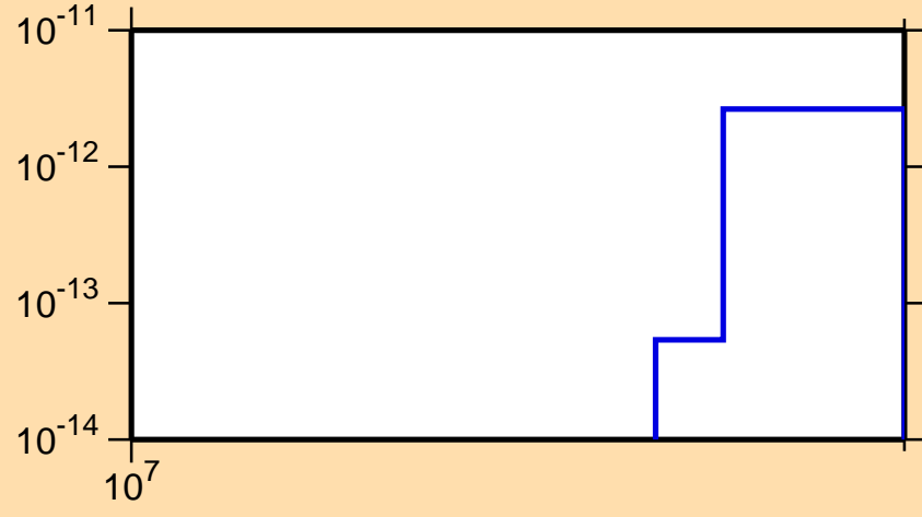
\sigma vs. E for ^{251}\text{Bk}(n,\text{He3})
