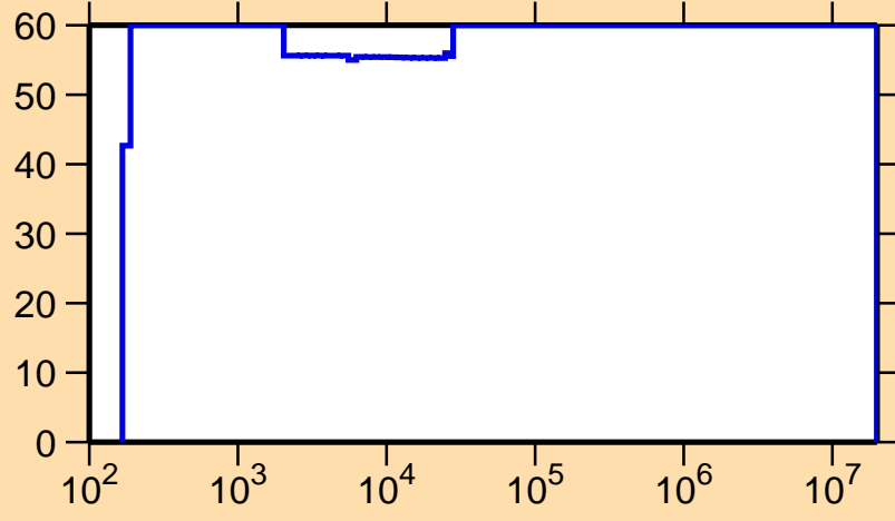
\Delta\sigma/\sigma vs. E for ^{251}\text{Bk}(n,\gamma)
