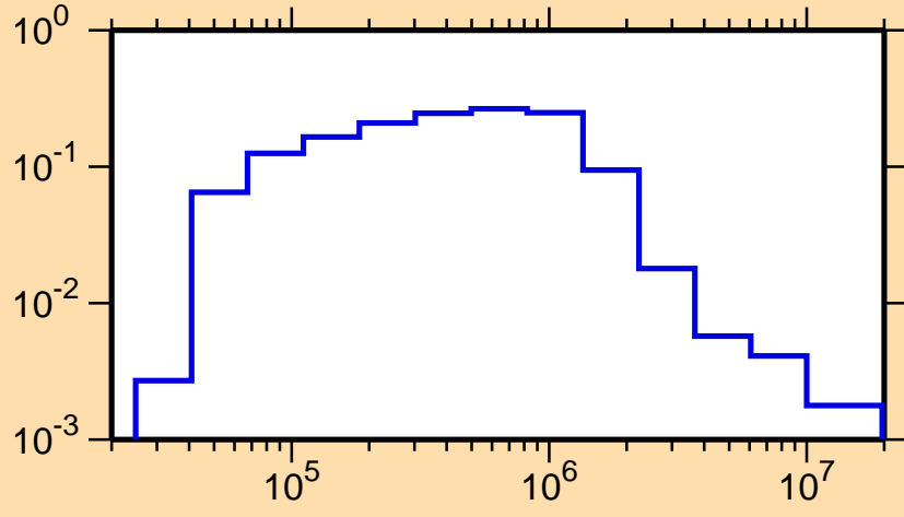
\sigma vs. E for ^{251}\text{Bk}(n,n_2)
