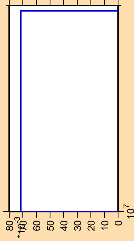
\Delta\sigma/\sigma vs. E for ^{251}\text{Bk} (mt 11)
