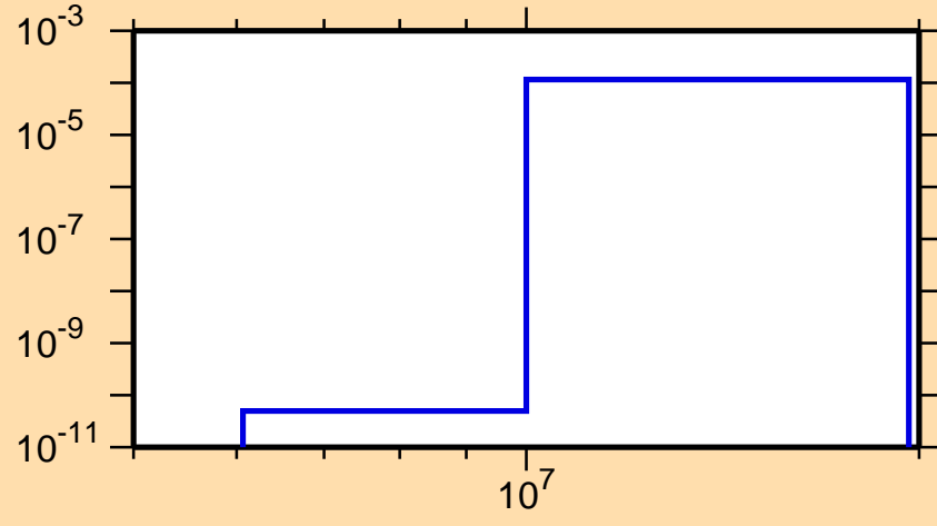
\sigma vs. E for ^{251}\text{Bk}(n,np)
