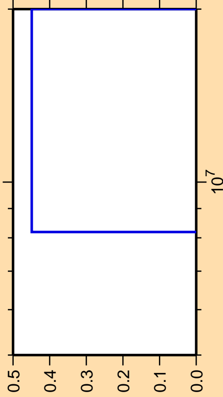
\Delta\sigma/\sigma vs. E for ^{251}\text{Bk}(\text{mt } 45)
