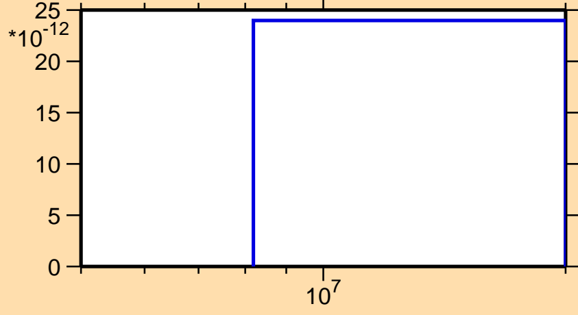
\sigma vs. E for ^{251}\text{Bk}(n,p\alpha)
