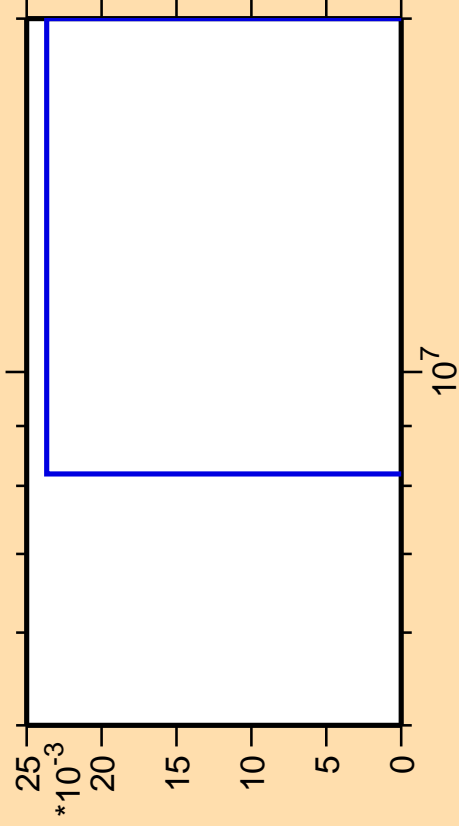
\Delta\sigma/\sigma vs. E for ^{251}\text{Bk} (mt 42)
