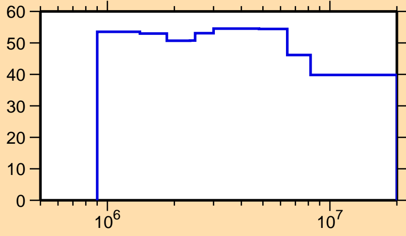
\Delta\sigma/\sigma vs. E for ^{251}\text{Bk}(n,n\text{cont.})
