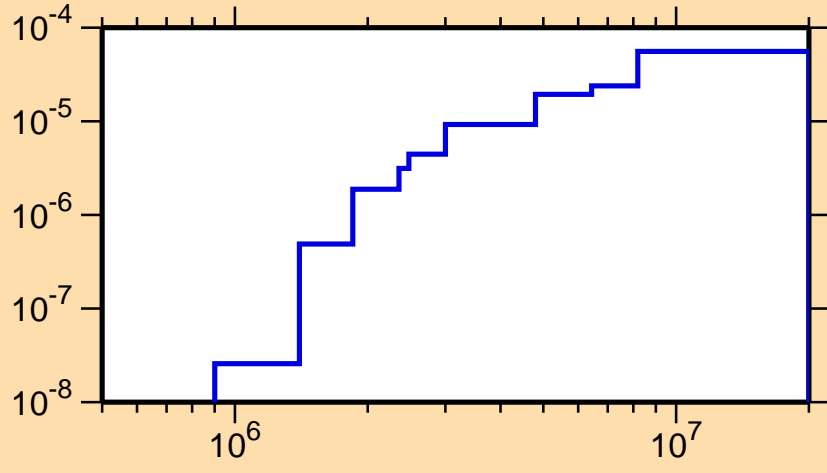
\sigma vs. E for ^{251}\text{Bk}(n,n\alpha)
