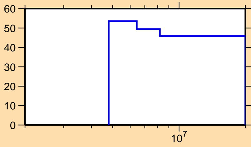
\Delta\sigma/\sigma vs. E for ^{251}\text{Bk}(n,2n)
