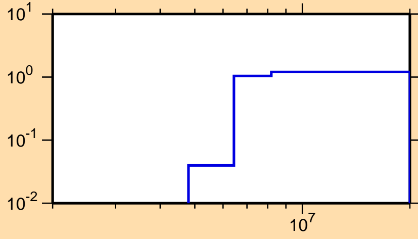
\sigma vs. E for ^{251}\text{Bk}(n,2n)
