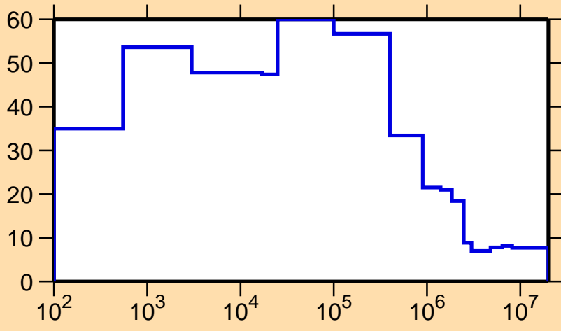
\Delta\sigma/\sigma vs. E for ^{251}\text{Bk}(n,\text{nonel.})
