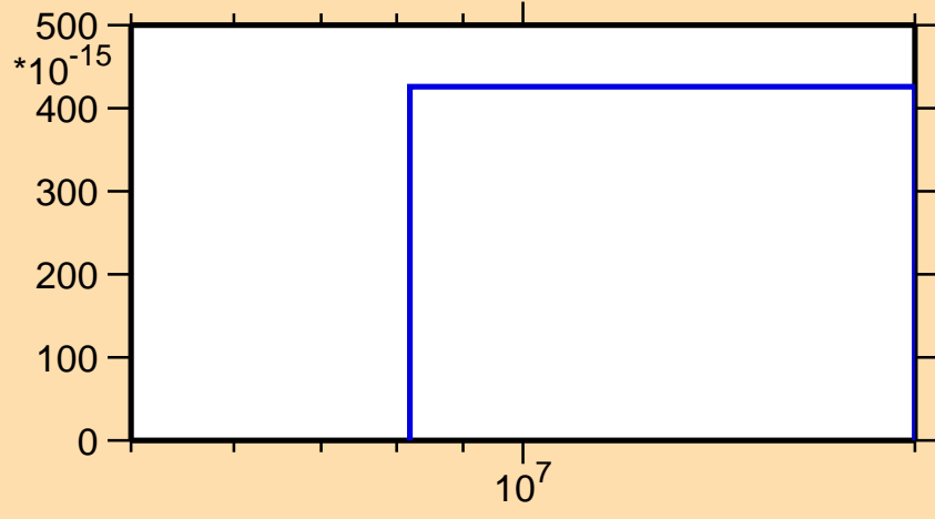
\sigma vs. E for ^{251}\text{Bk}(\text{mt117})
