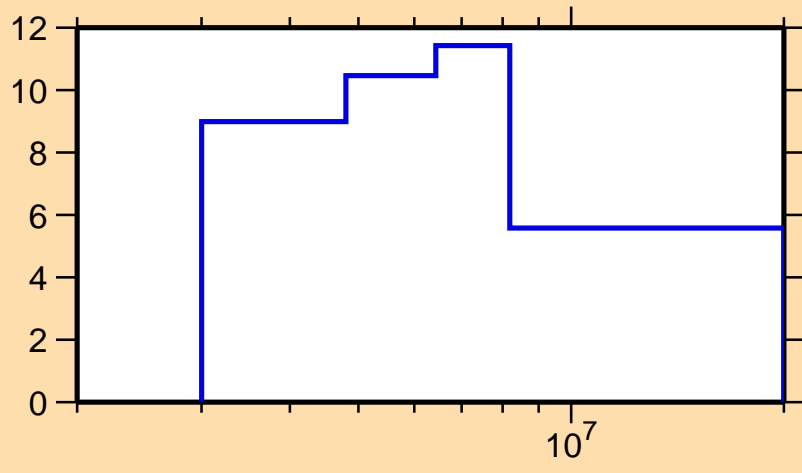
\Delta\sigma/\sigma vs. E for ^{251}\text{Bk}(n,\text{el.})
