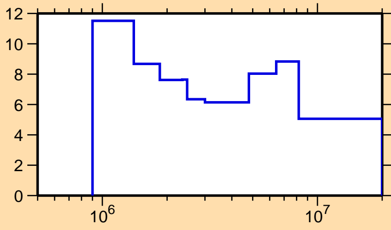
\Delta\sigma/\sigma vs. E for ^{251}\text{Bk}(n,\text{tot.})
