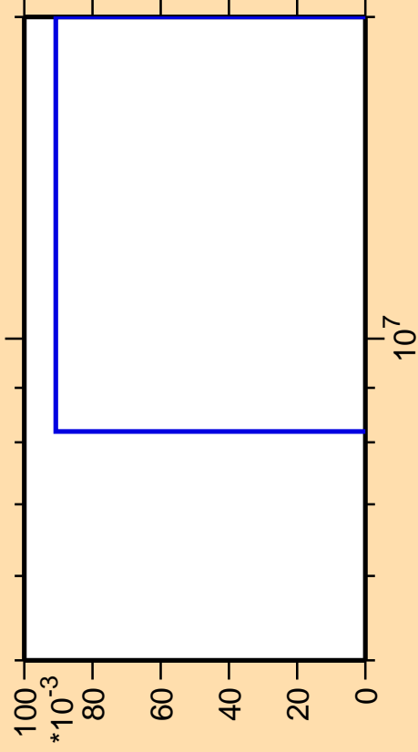
\Delta\sigma/\sigma vs. E for ^{251}\text{Bk}(\text{mt } 11)
