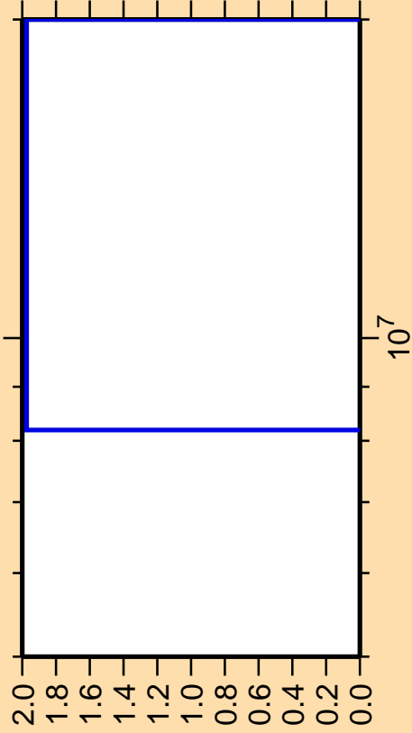
\Delta\sigma/\sigma vs. E for ^{251}\text{Bk}(\text{mt117})
