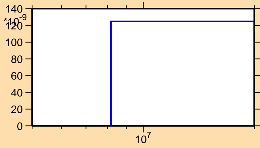
\sigma vs. E for ^{251}\text{Bk}(n,3n\alpha)
