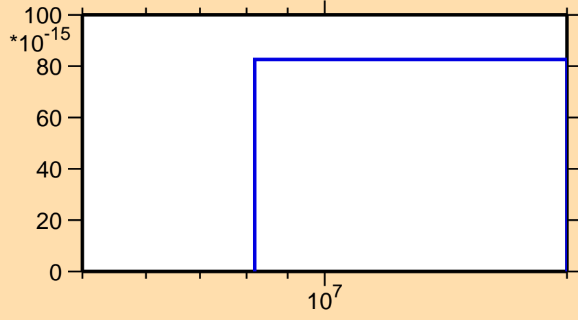
\sigma vs. E for ^{251}\text{Bk}(\text{mt } 45)
