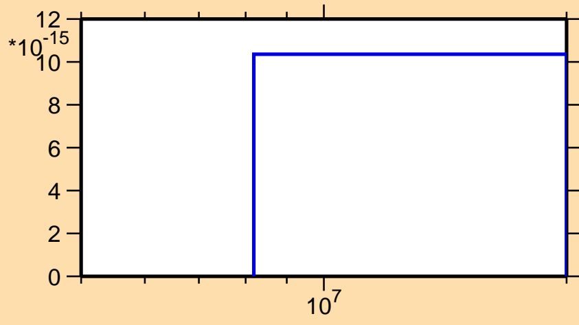
\sigma vs. E for ^{251}\text{Bk} (mt 42)
