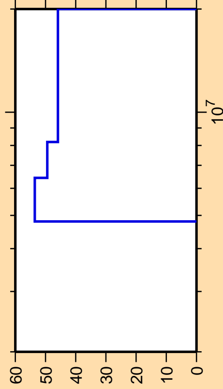
\Delta\sigma/\sigma vs. E for ^{251}\text{Bk}(n,2n)
