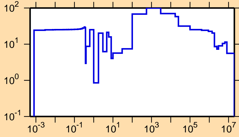
\Delta\sigma/\sigma vs. E for ^{251}\text{Bk}(n,el.)
