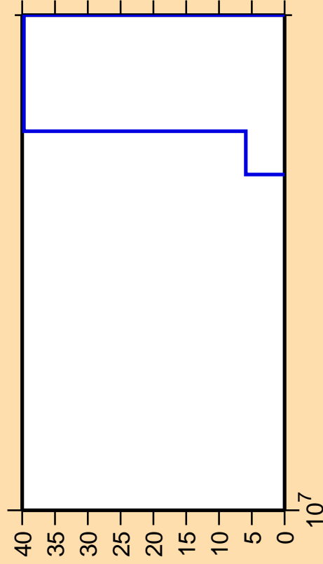
\Delta\sigma/\sigma vs. E for ^{252}\text{Bk} (mt 45)
