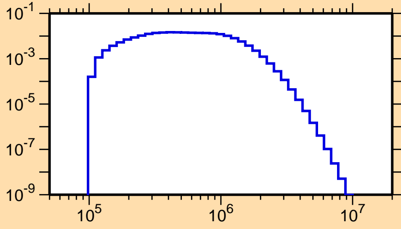
\sigma vs. E for ^{252}\text{Bk}(n,n_1)
