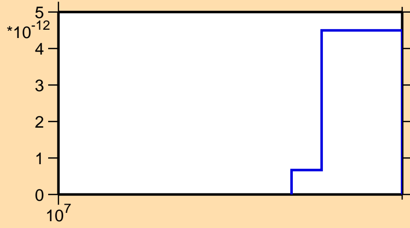
\sigma vs. E for ^{252}\text{Bk} (mt 45)
