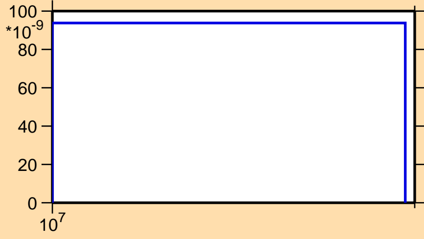
\sigma vs. E for ^{252}\text{Bk}(n,2np)
