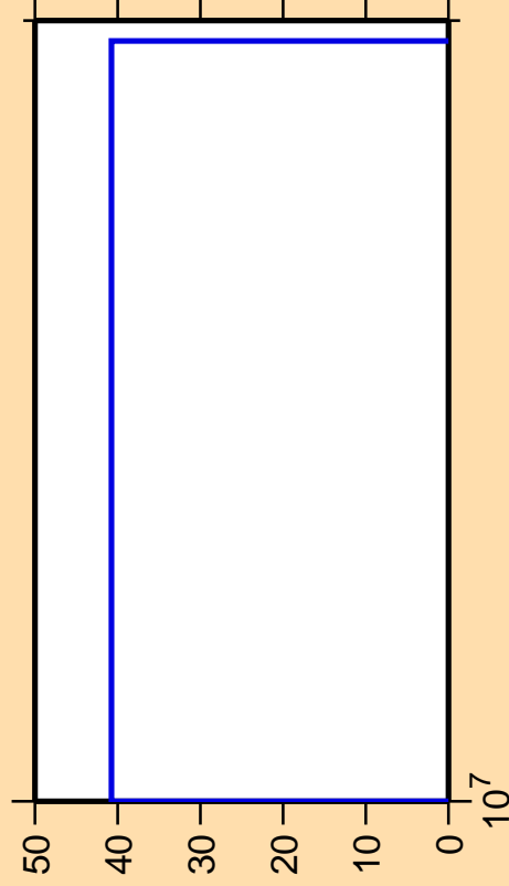
\Delta\sigma/\sigma vs. E for ^{252}\text{Bk}(n,nd)
