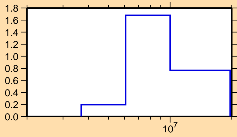
\sigma vs. E for ^{252}\text{Bk}(n,2n)
