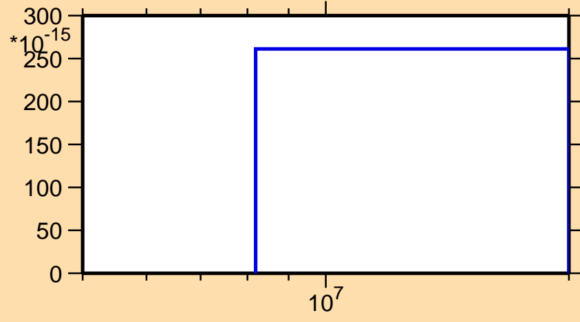
\sigma vs. E for ^{252}\text{Bk}(\text{mt } 11)
