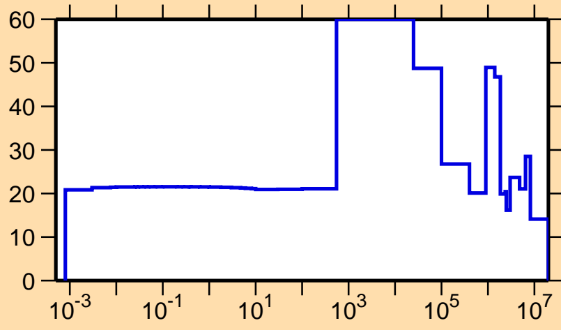
\Delta\sigma/\sigma vs. E for ^{252}\text{Bk}(n,el.)
