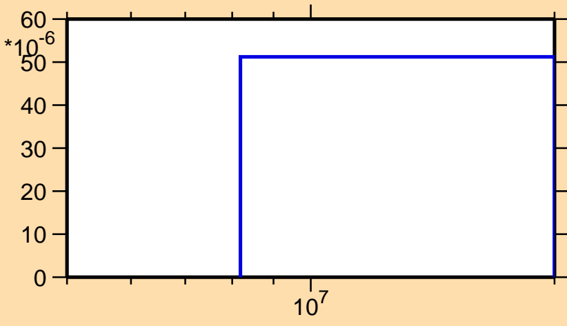
\sigma vs. E for ^{252}\text{Bk}(n,np)
