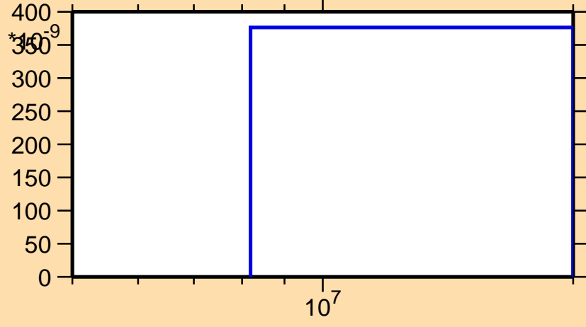
\sigma vs. E for ^{252}\text{Bk}(n,nd)
