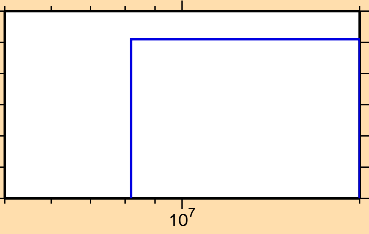
\sigma vs. E for ^{252}\text{Bk} (mt 42)
