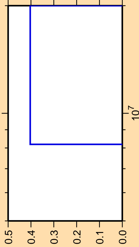
\Delta\sigma/\sigma vs. E for ^{252}\text{Bk}(\text{mt } 11)
