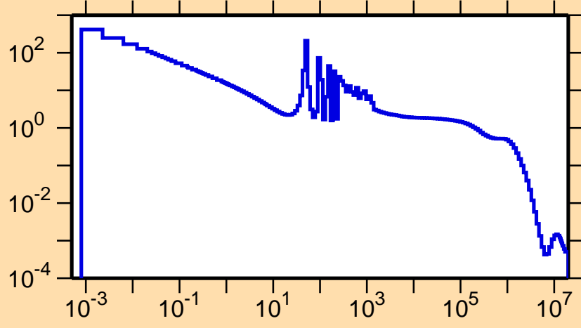
\sigma vs. E for ^{253}\text{Bk}(n,\gamma)
