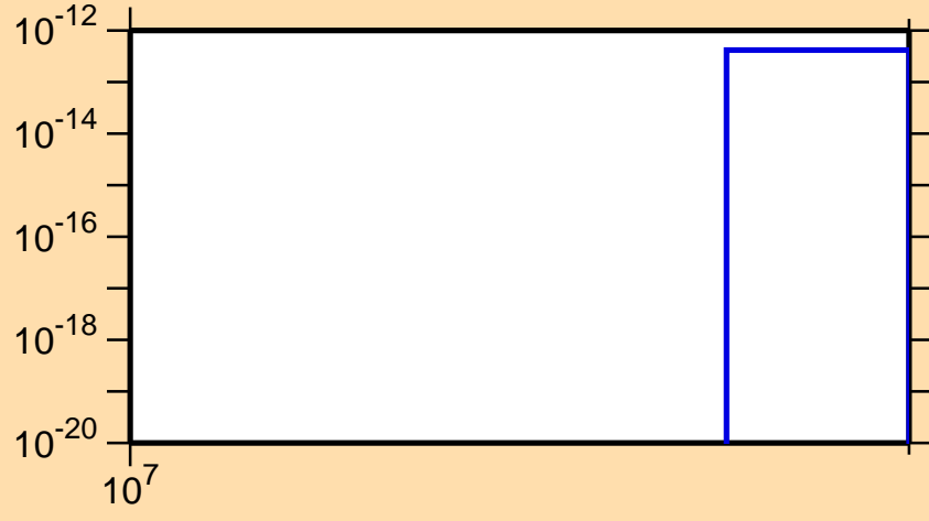
\sigma vs. E for ^{253}\text{Bk} (mt 42)
