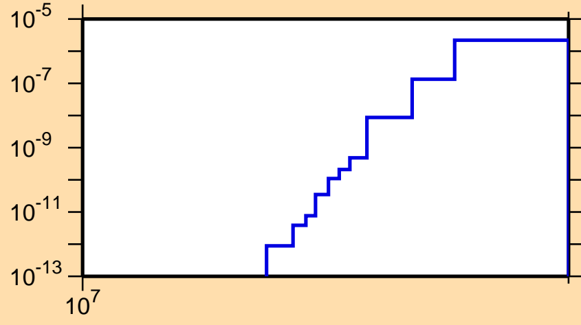
\sigma vs. E for ^{253}\text{Bk}(n,nd)
