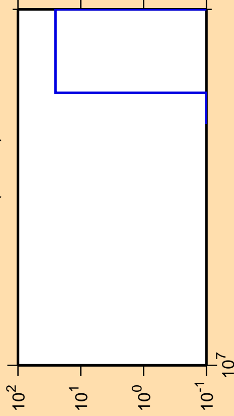
\Delta\sigma/\sigma vs. E for ^{253}\text{Bk} (mt 11)
