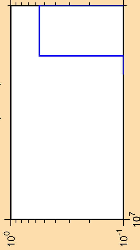
\Delta\sigma/\sigma vs. E for ^{253}\text{Bk} (mt 42)
