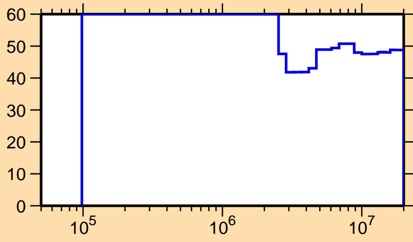
\Delta\sigma/\sigma vs. E for ^{253}\text{Bk}(n,n_1)
