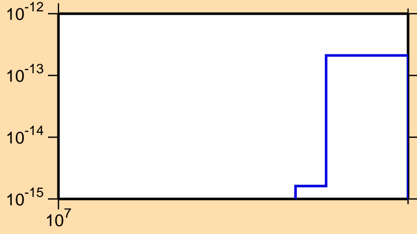
\sigma vs. E for ^{253}\text{Bk}(n,\text{He3})
