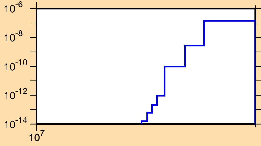
\sigma vs. E for ^{253}\text{Bk}(n,2np)
