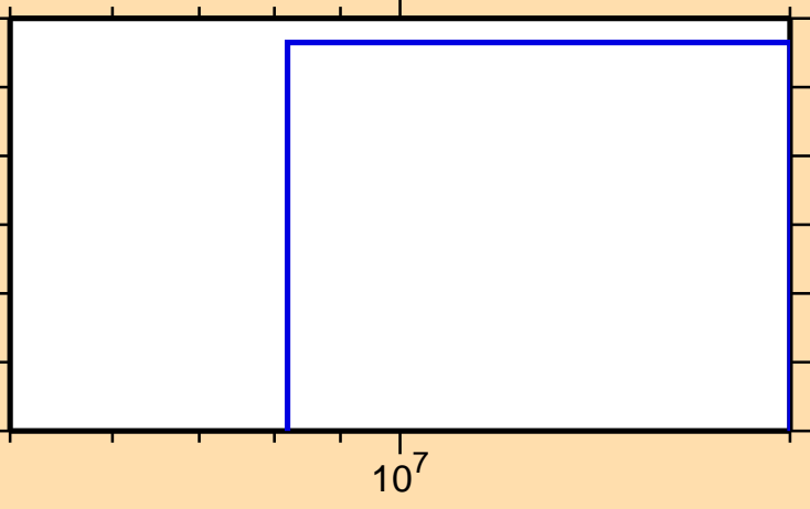
\sigma vs. E for ^{253}\text{Bk}(n,nt)
