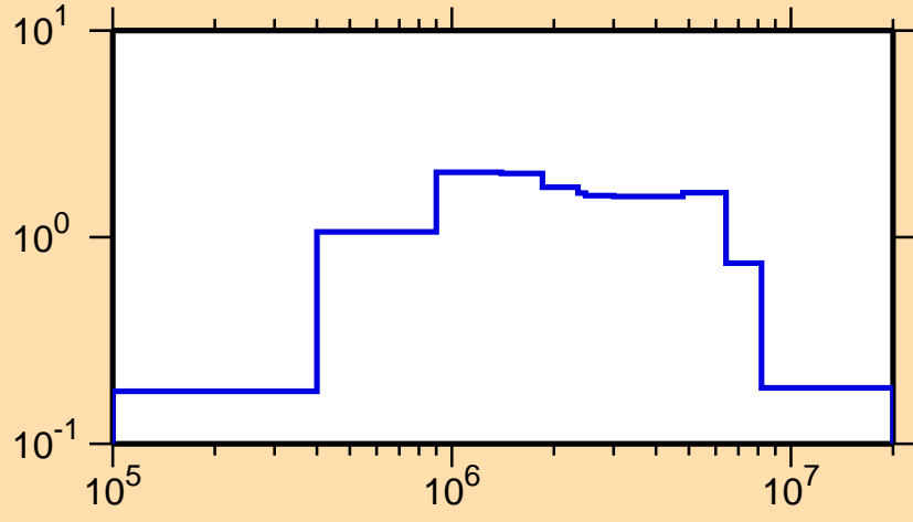
\sigma vs. E for ^{253}\text{Bk}(n,n\text{cont.})
