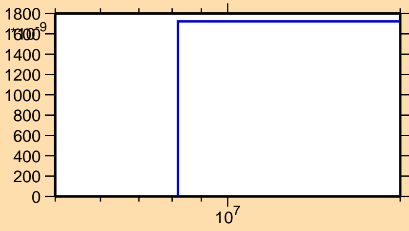
\sigma vs. E for ^{253}\text{Bk}(n,3n\alpha)
