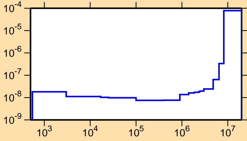
\sigma vs. E for ^{253}\text{Bk}(n,\alpha)
