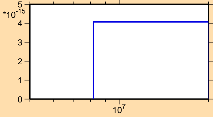
\sigma vs. E for ^{253}\text{Bk} (mt 45)
