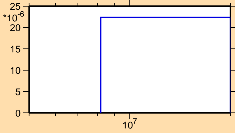
\sigma vs. E for ^{253}\text{Bk}(n,np)
