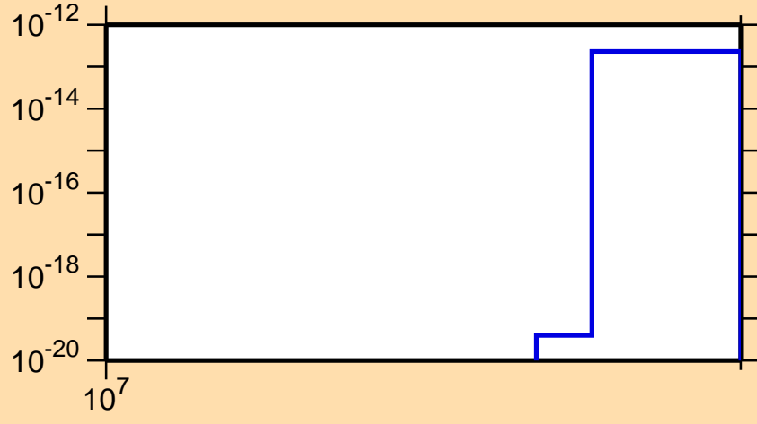
\sigma vs. E for ^{254}\text{Bk} (mt 42)
