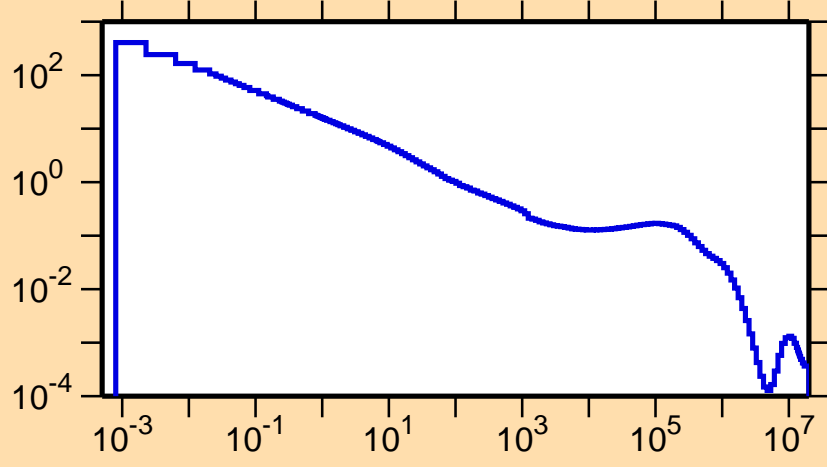
\sigma vs. E for ^{254}\text{Bk}(n,\gamma)
