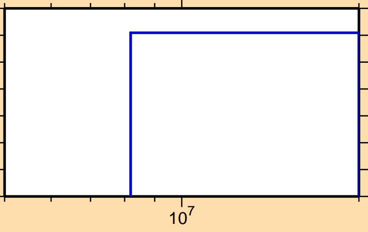
\sigma vs. E for ^{254}\text{Bk} (mt 11)
