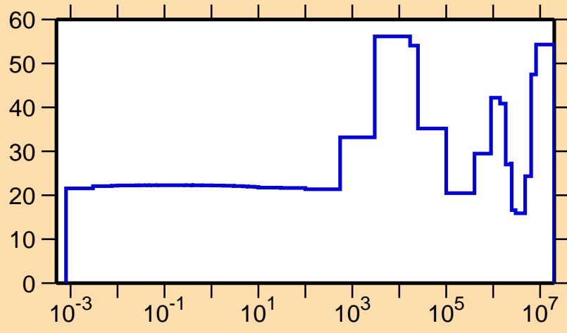
\Delta\sigma/\sigma vs. E for ^{254}\text{Bk}(n,el.)
