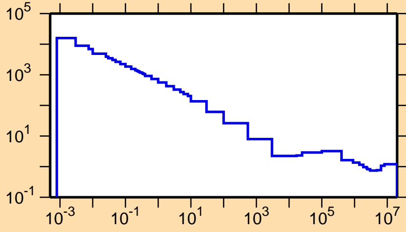
\sigma vs. E for ^{254}\text{Bk}(n,f)
