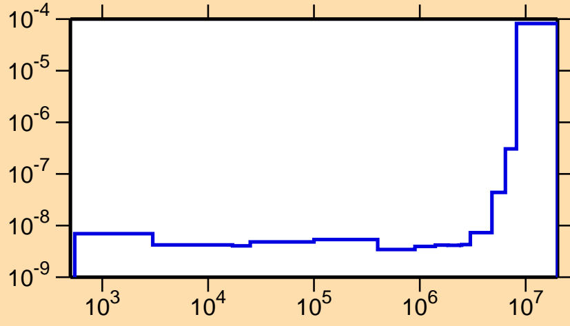
\sigma vs. E for ^{254}\text{Bk}(n,\alpha)
