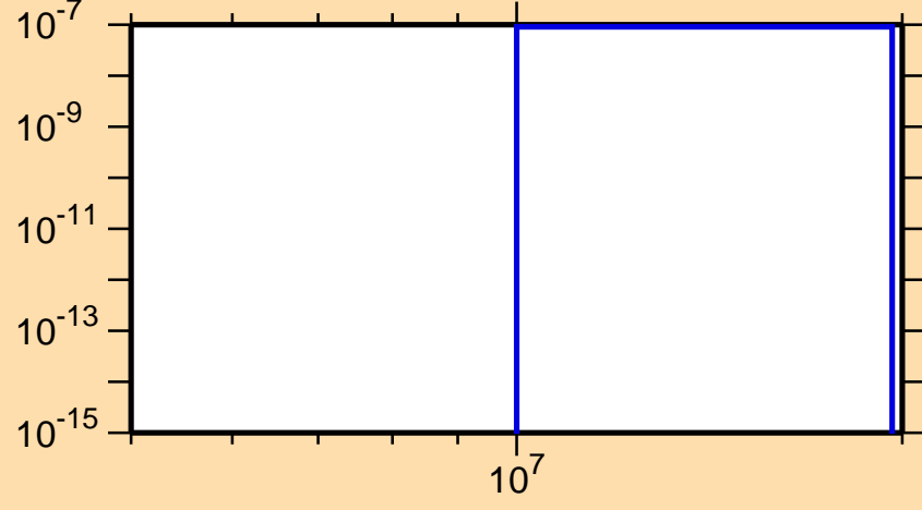
\sigma vs. E for ^{70}\text{Br} (mt 34)
