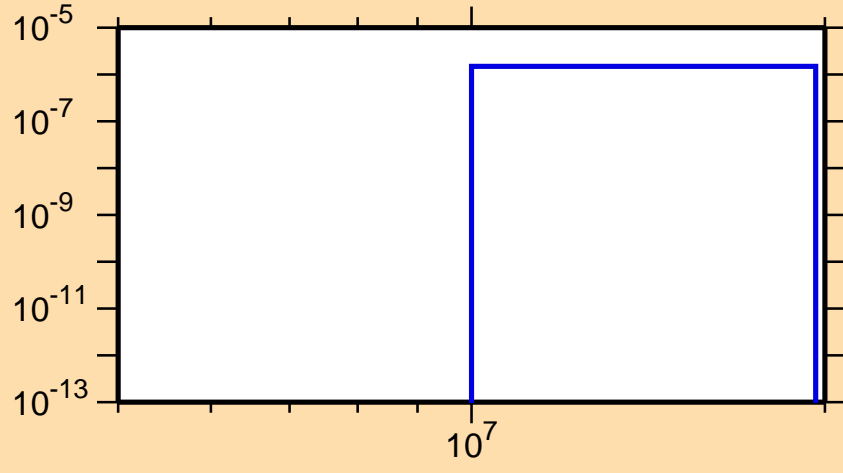
\sigma vs. E for ^{70}\text{Br}(n,nd)
