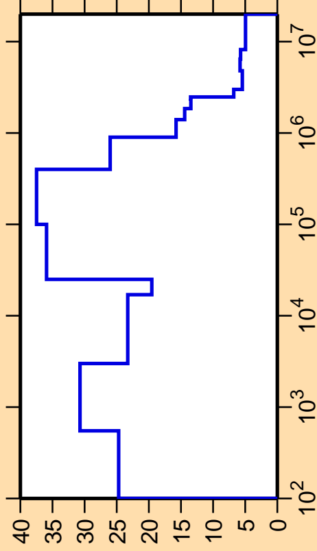
\Delta\sigma/\sigma vs. E for ^{70}\text{Br}(n,\text{nonel.})
