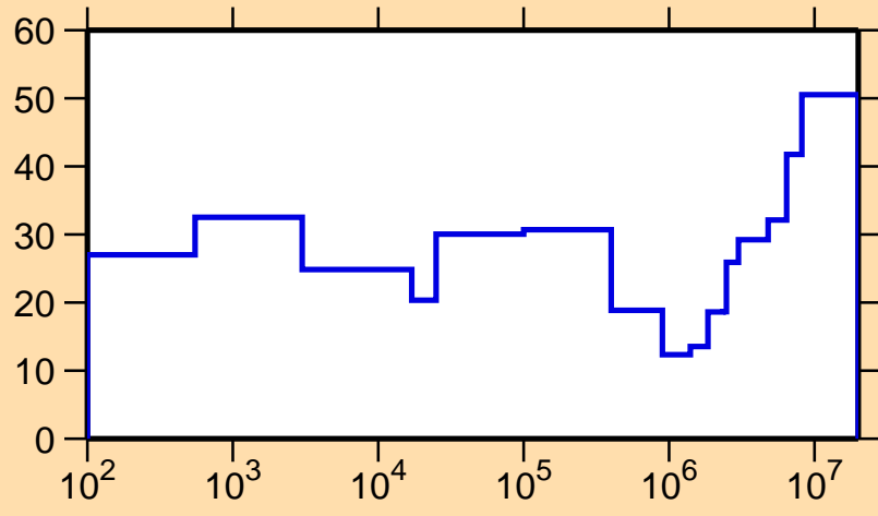
\Delta\sigma/\sigma vs. E for ^{70}\text{Br}(n,p)
