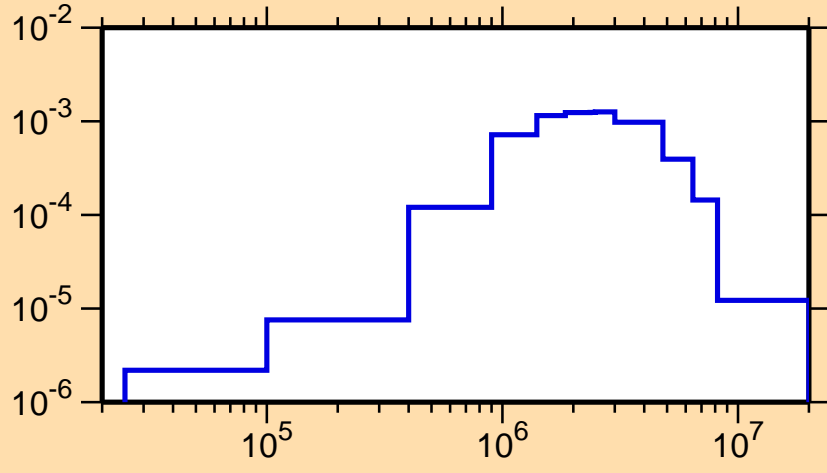
\sigma vs. E for ^{70}\text{Br}(n,n\text{cont.})
