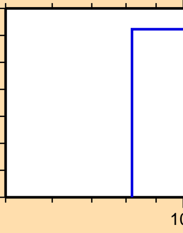
\sigma vs. E for ^{70}\text{Br}(n,2n\alpha)
