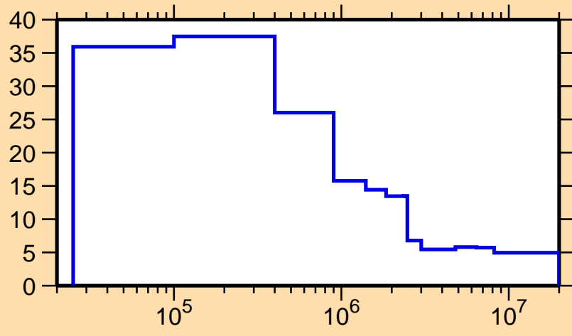
\Delta\sigma/\sigma vs. E for ^{70}\text{Br}(n,\text{nonel.})
