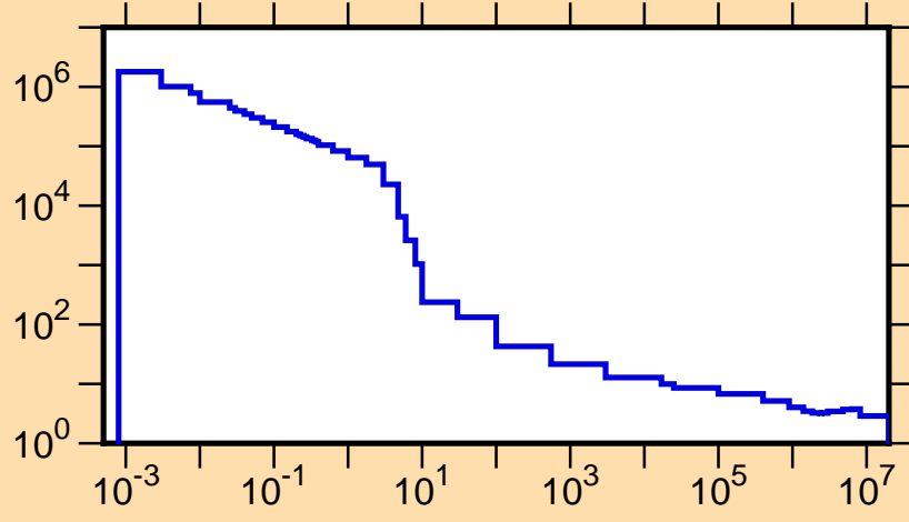
\sigma vs. E for ^{70}\text{Br}(n,\text{tot.})
