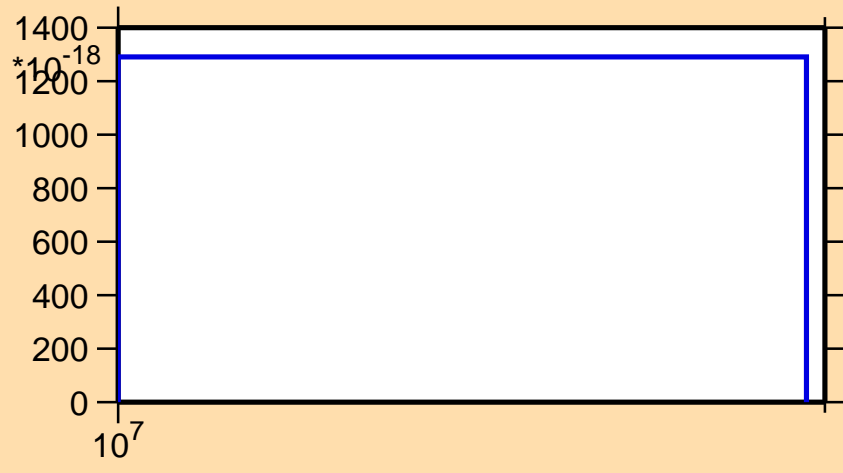
\sigma vs. E for ^{71}\text{Br}(n,nt)
