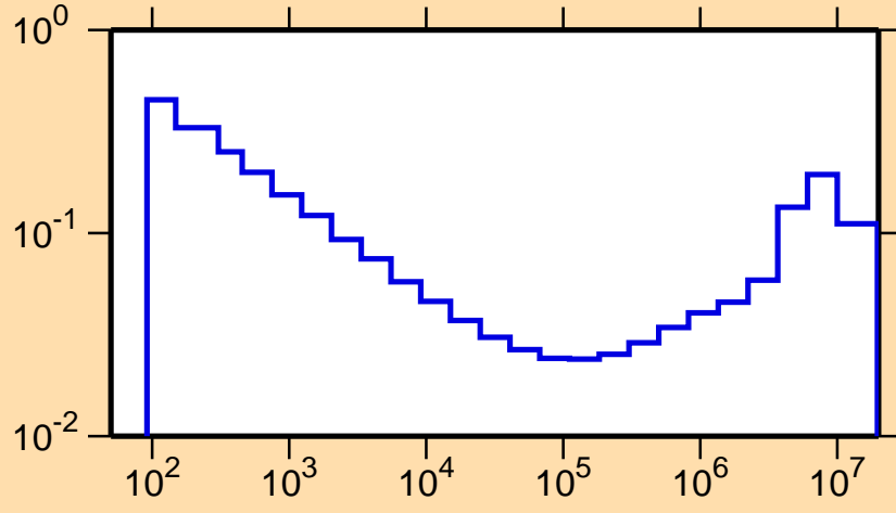
\sigma vs. E for ^{71}\text{Br}(n,\alpha)
