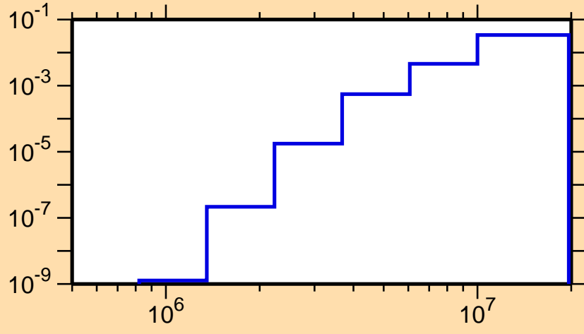
\sigma vs. E for ^{71}\text{Br}(n,d)
