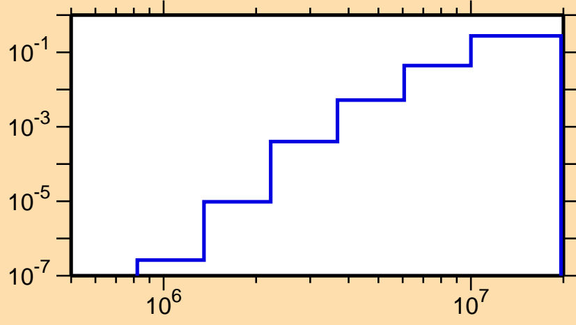
\sigma vs. E for ^{71}\text{Br}(n,p\alpha)
