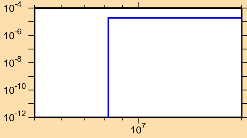
\sigma vs. E for ^{71}\text{Br}(\text{mt117})
