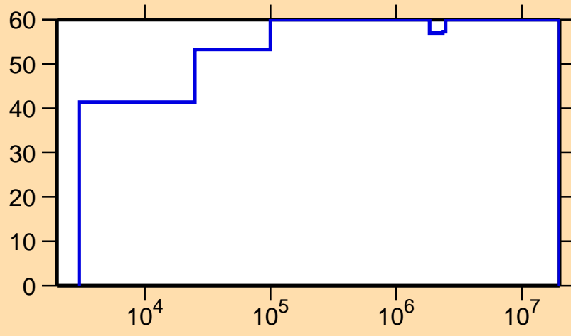
\Delta\sigma/\sigma vs. E for ^{71}\text{Br}(n,n_1)
