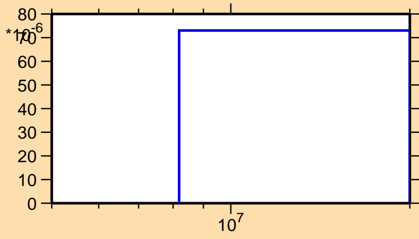
\sigma vs. E for ^{71}\text{Br} (mt 45)
