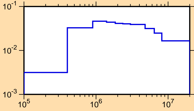
\sigma vs. E for ^{71}\text{Br}(n,n_2)
