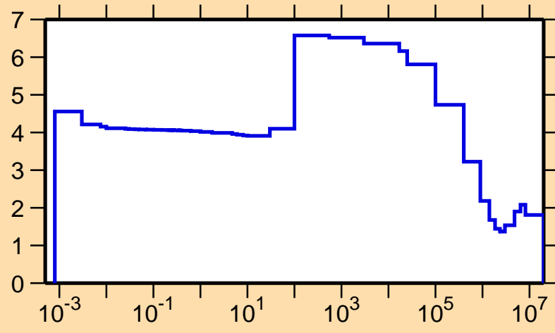
\sigma vs. E for ^{71}\text{Br}(n,\text{el.})
