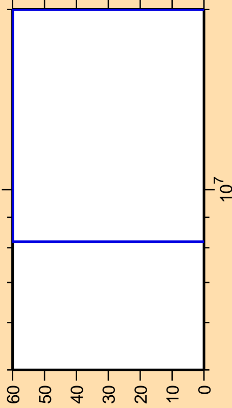
\Delta\sigma/\sigma vs. E for ^{71}\text{Br}(n,2n)
