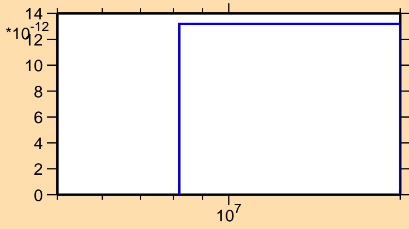
\sigma vs. E for ^{71}\text{Br} (mt 34)
