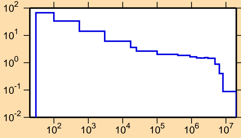
\sigma vs. E for ^{71}\text{Br}(n,p)
