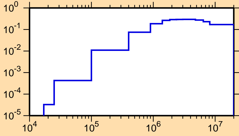
\sigma vs. E for ^{71}\text{Br}(n,\text{inel.})
