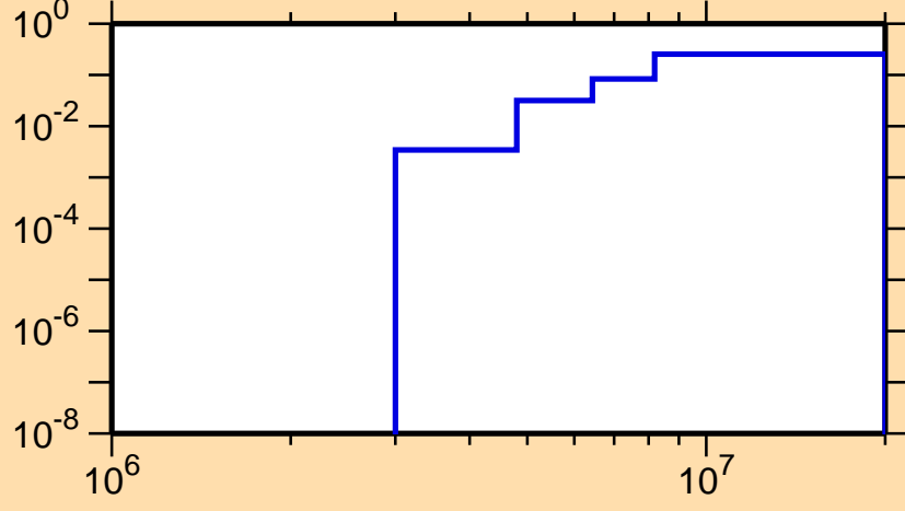
\sigma vs. E for ^{71}\text{Br}(n,np)
