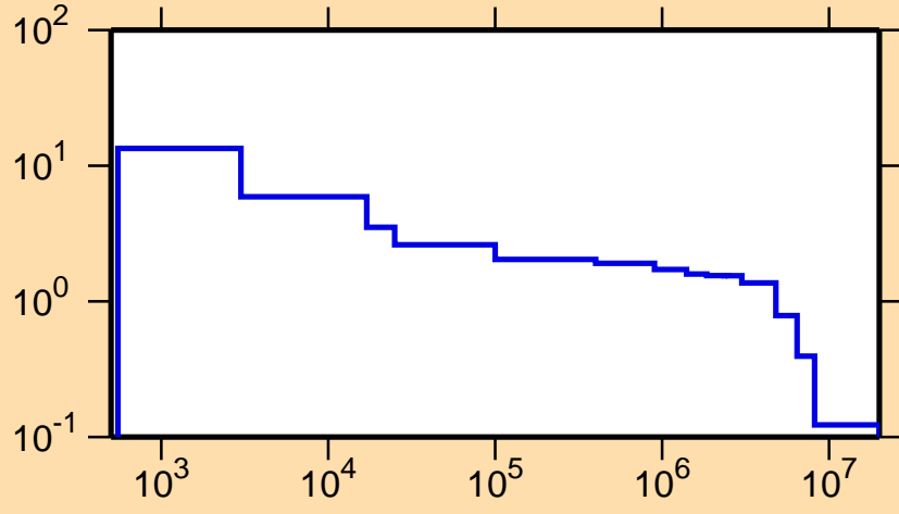
\sigma vs. E for ^{72}\text{Br}(n,p)
