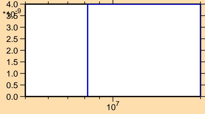
\sigma vs. E for ^{72}\text{Br} (mt 34)
